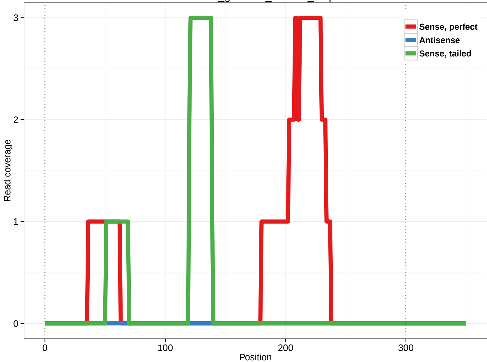
rheMac3_genscan_chr7.94_5.3p
