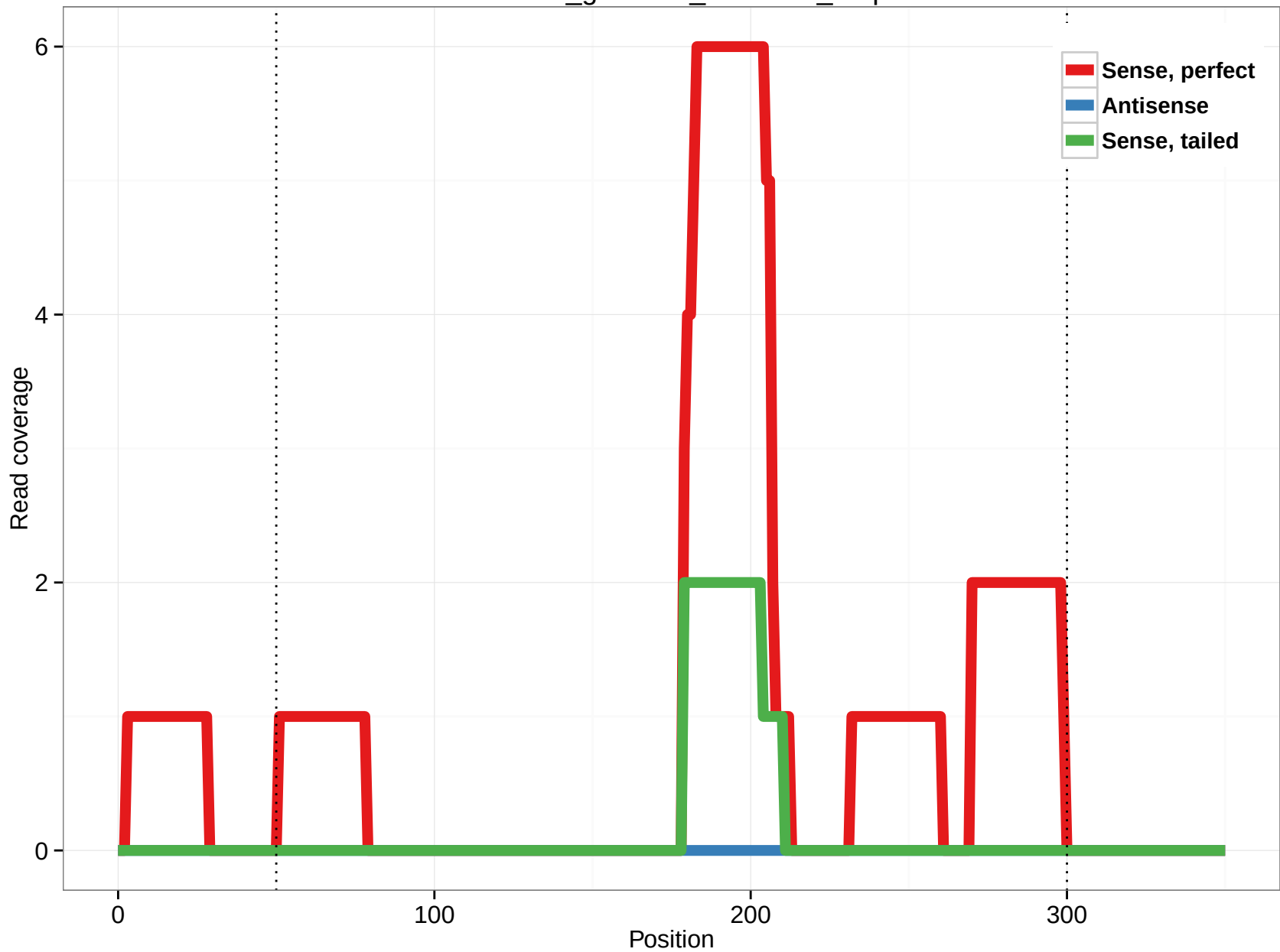
rheMac3_genscan_chr7.948_2.5p
