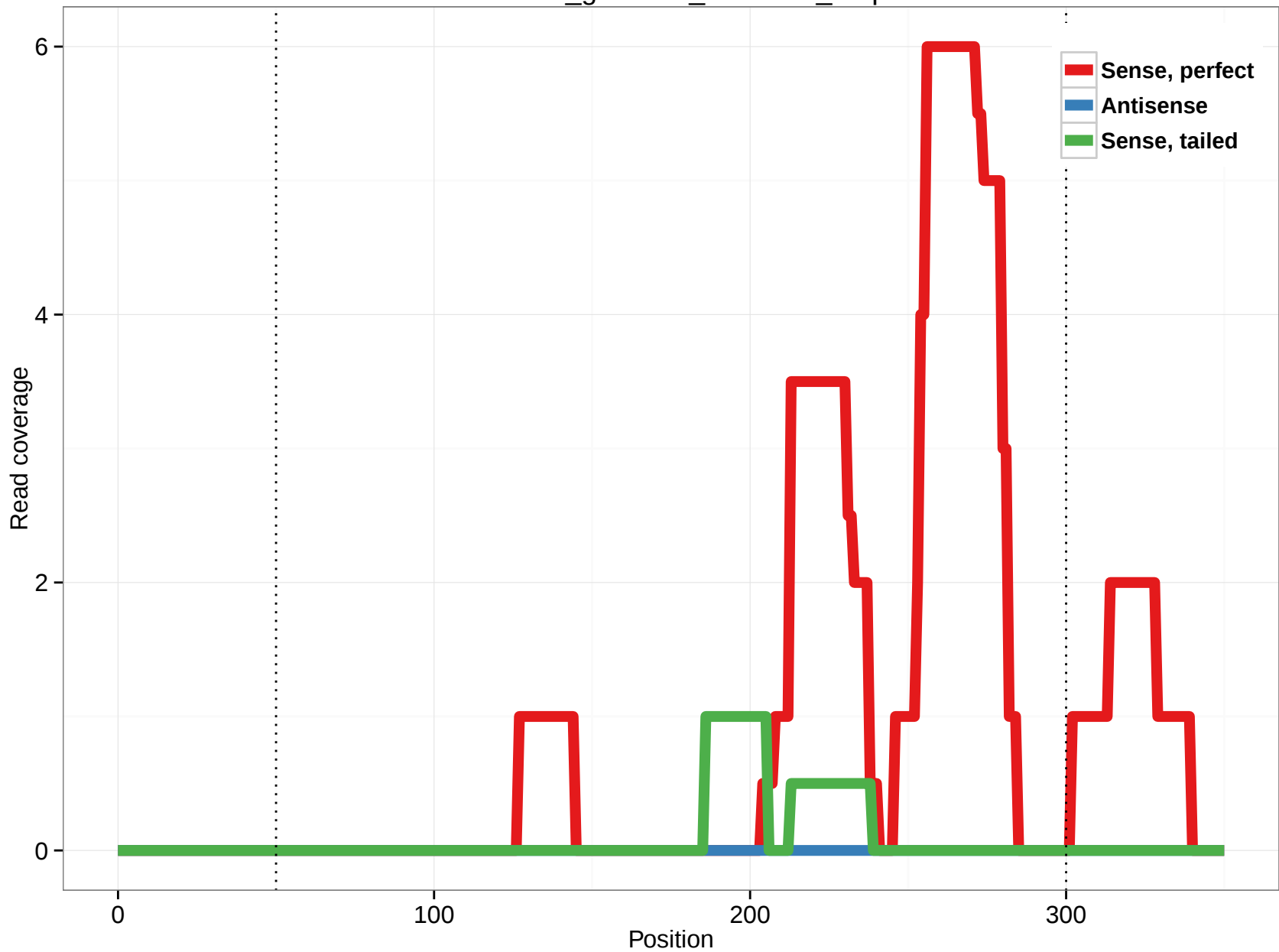
rheMac3_genscan_chr7.943_3.3p
