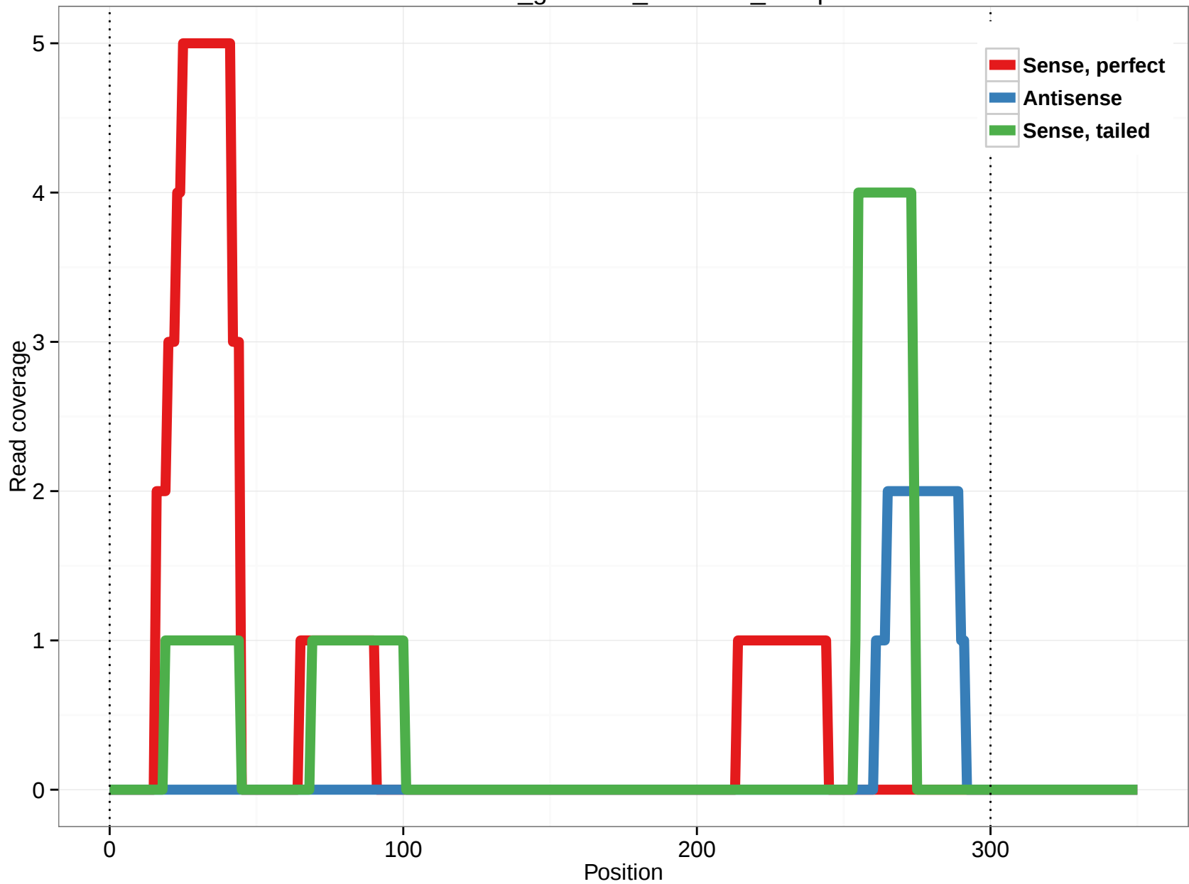
rheMac3_genscan_chr7.900_15.3p
