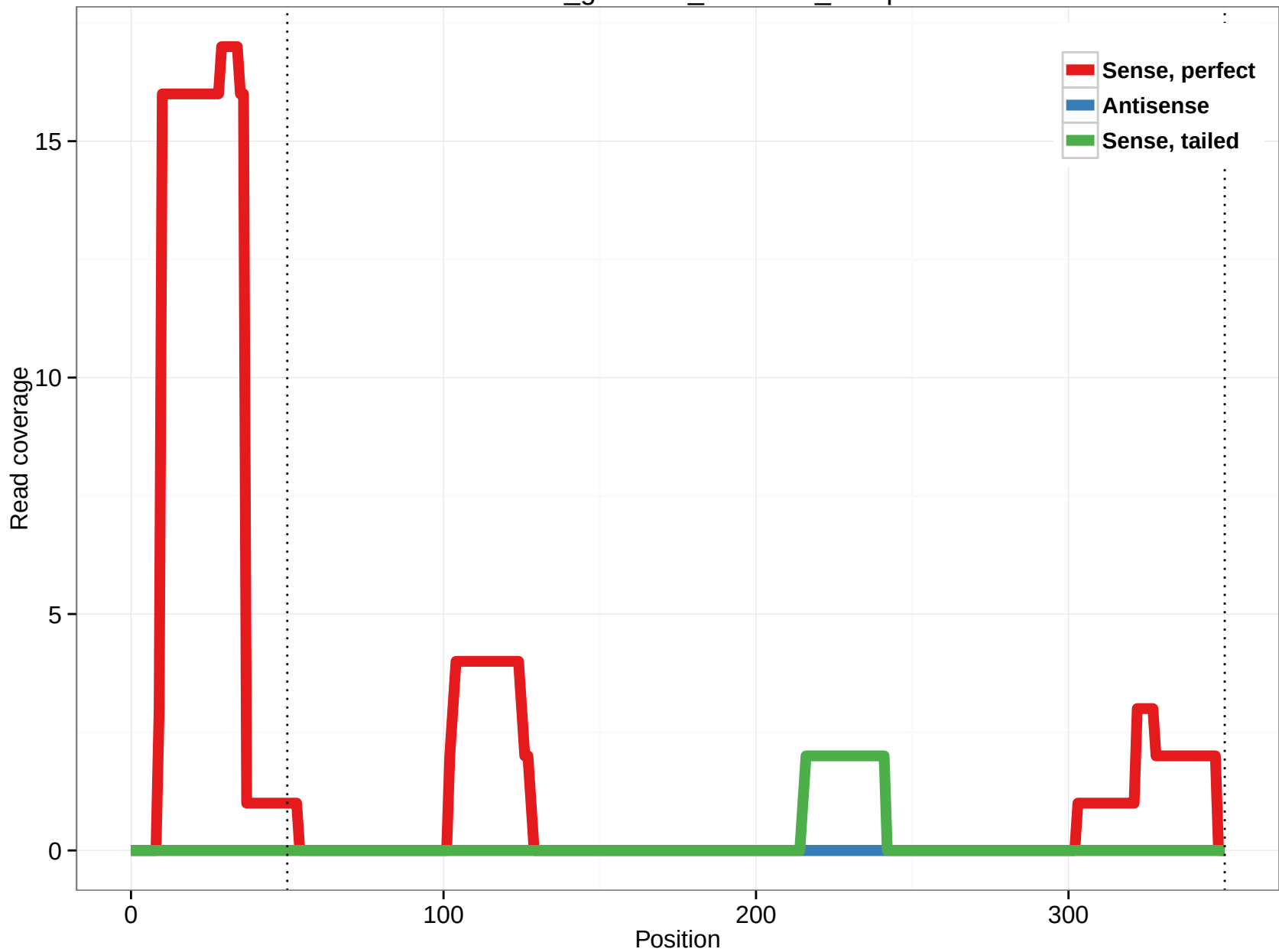
rheMac3_genscan_chr7.842_46.5p
