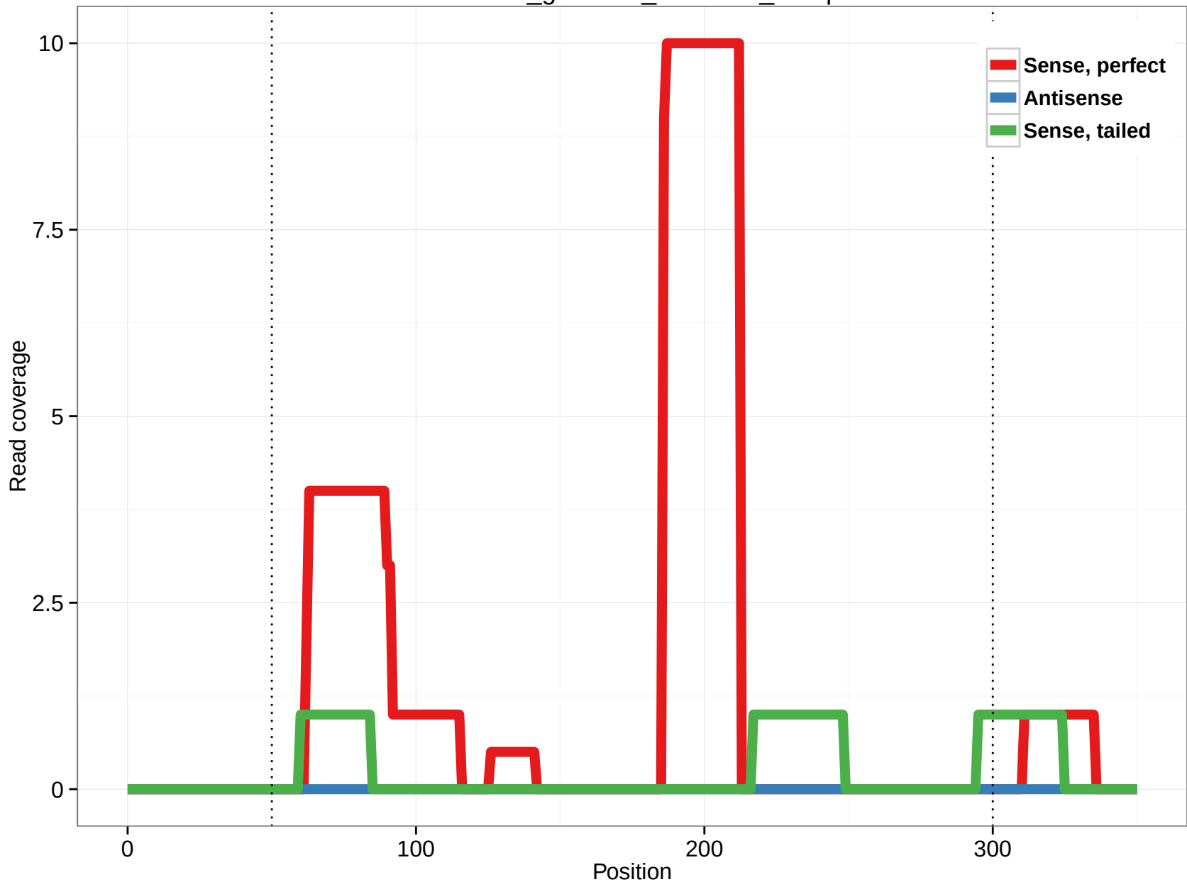
rheMac3_genscan_chr7.842_46.3p
