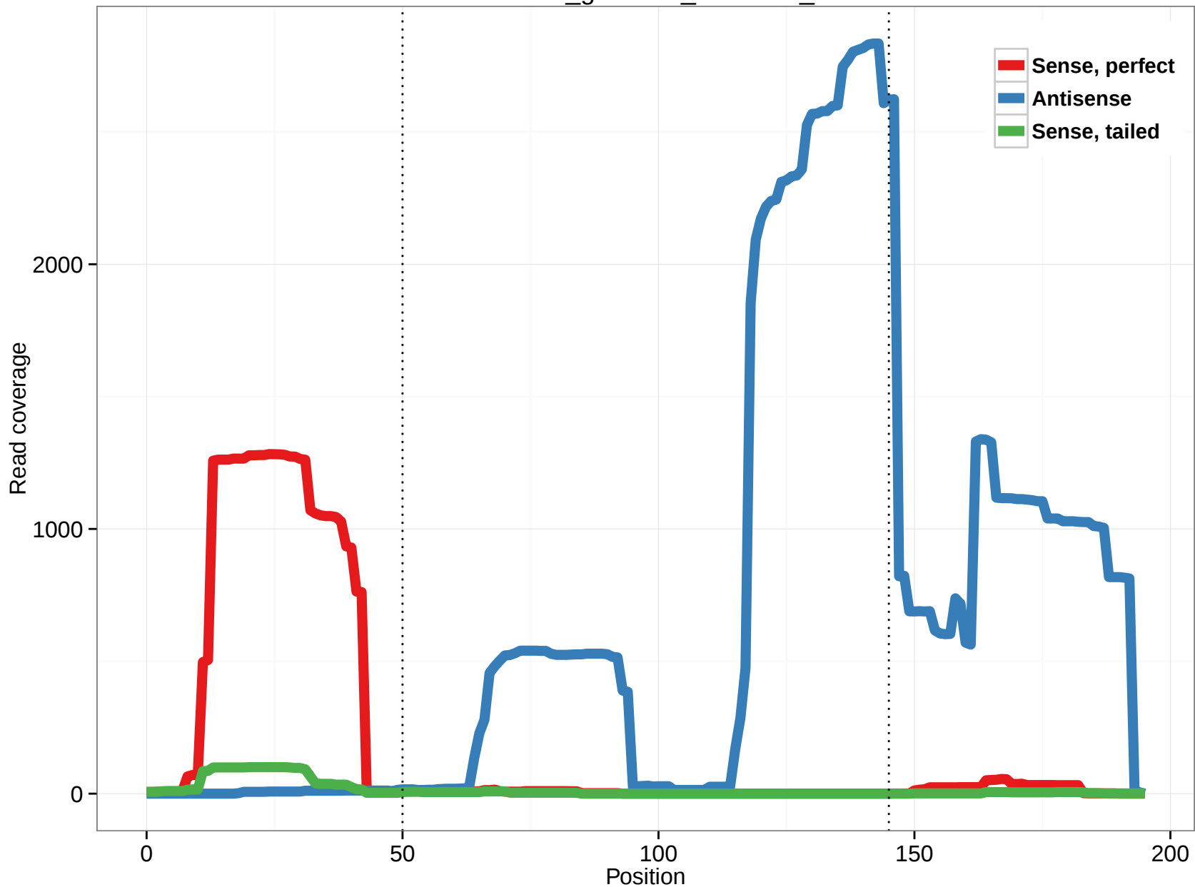
rheMac3_genscan_chr7.829_9
