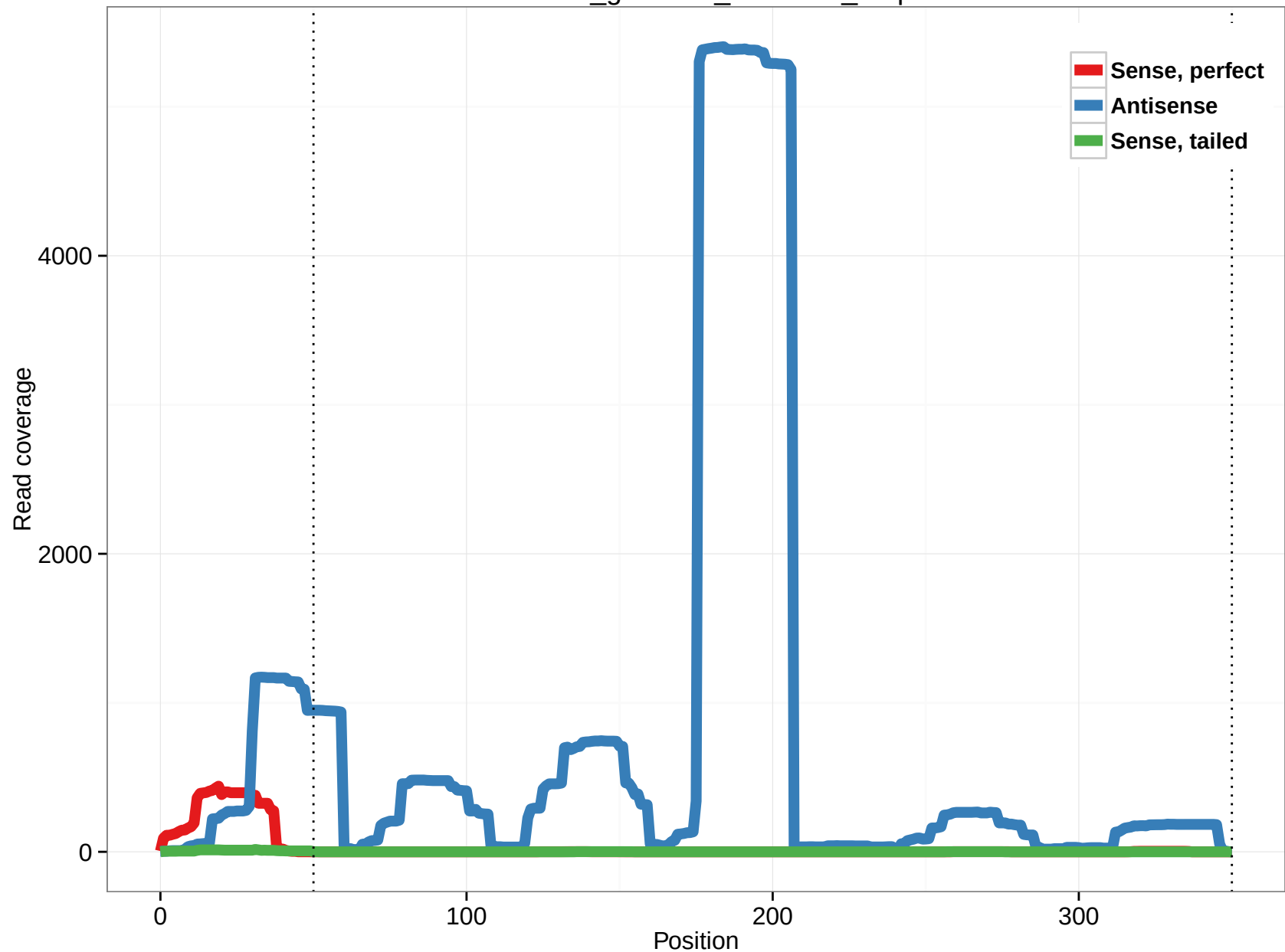
rheMac3_genscan_chr7.829_7.5p
