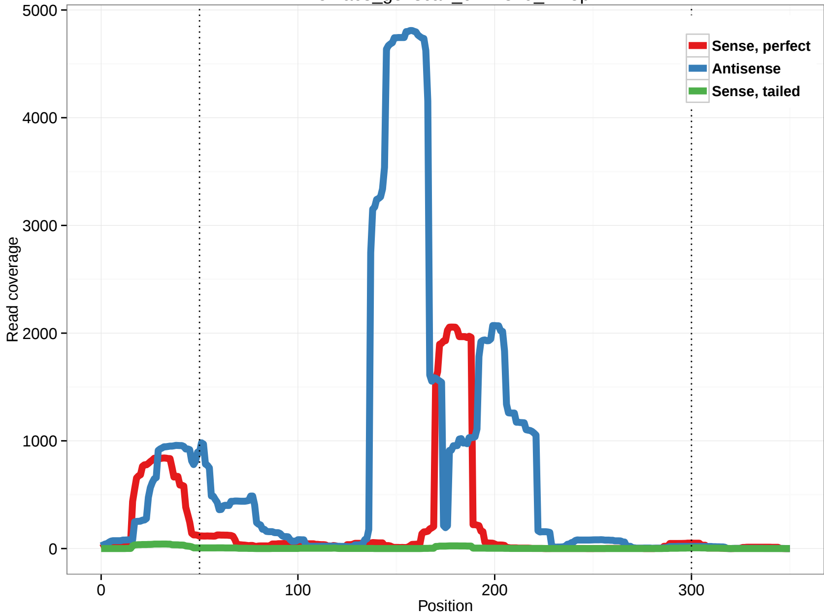
rheMac3_genscan_chr7.829_24.5p
