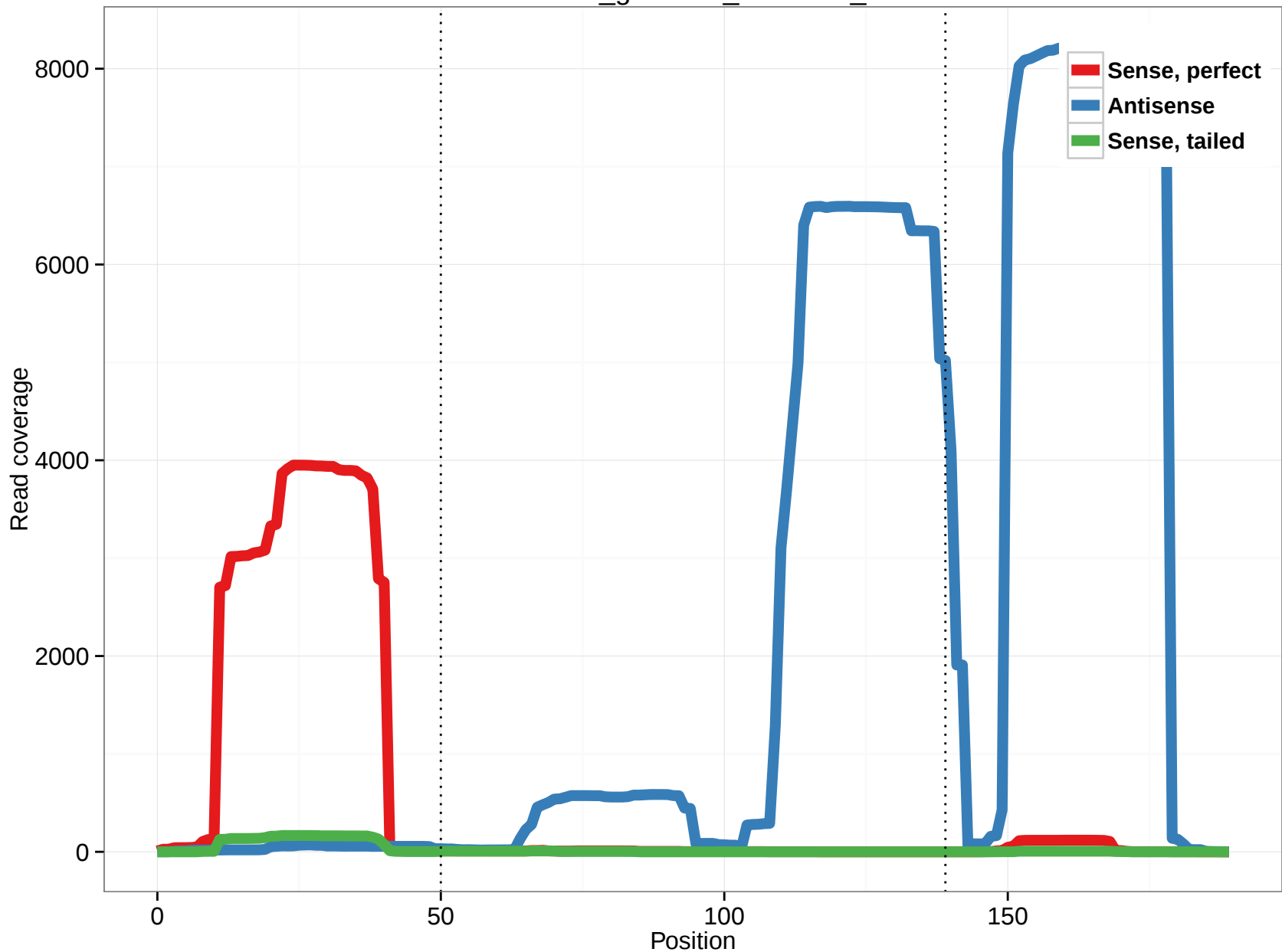
rheMac3_genscan_chr7.829_17
