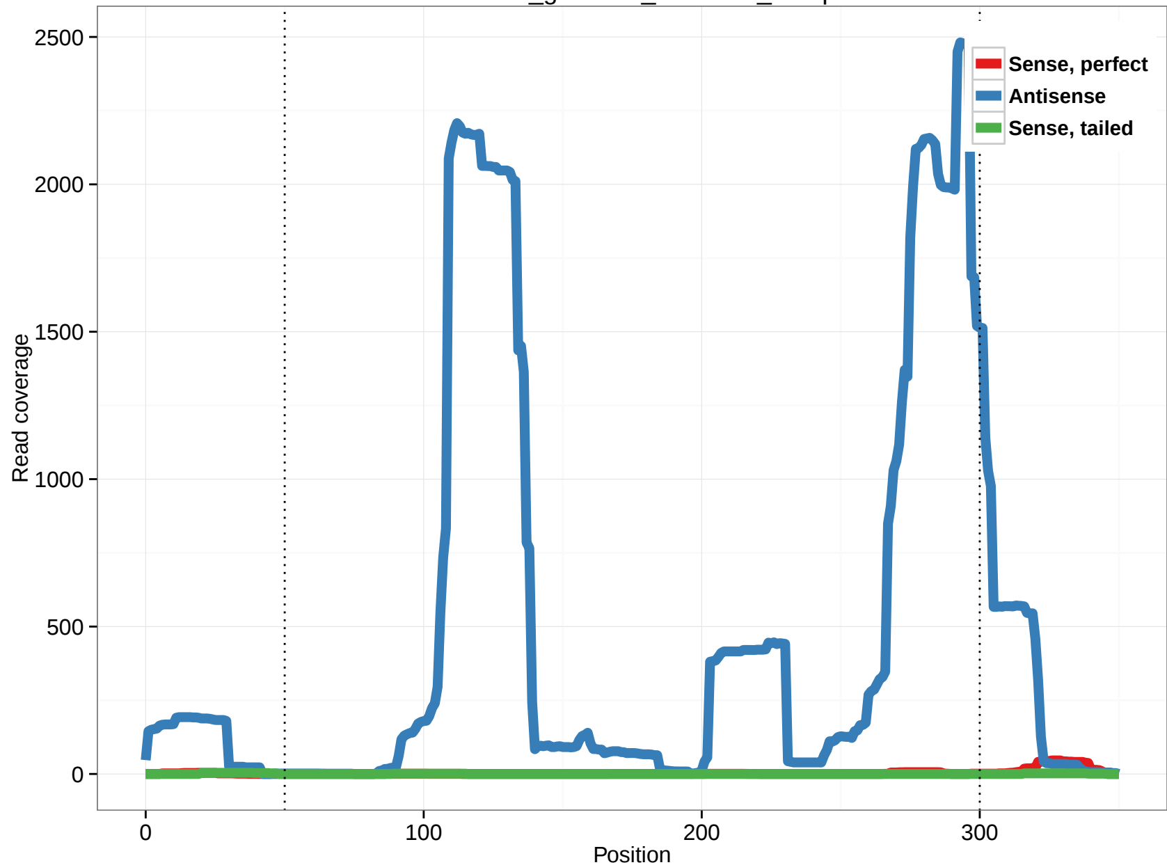
rheMac3_genscan_chr7.829_15.3p
