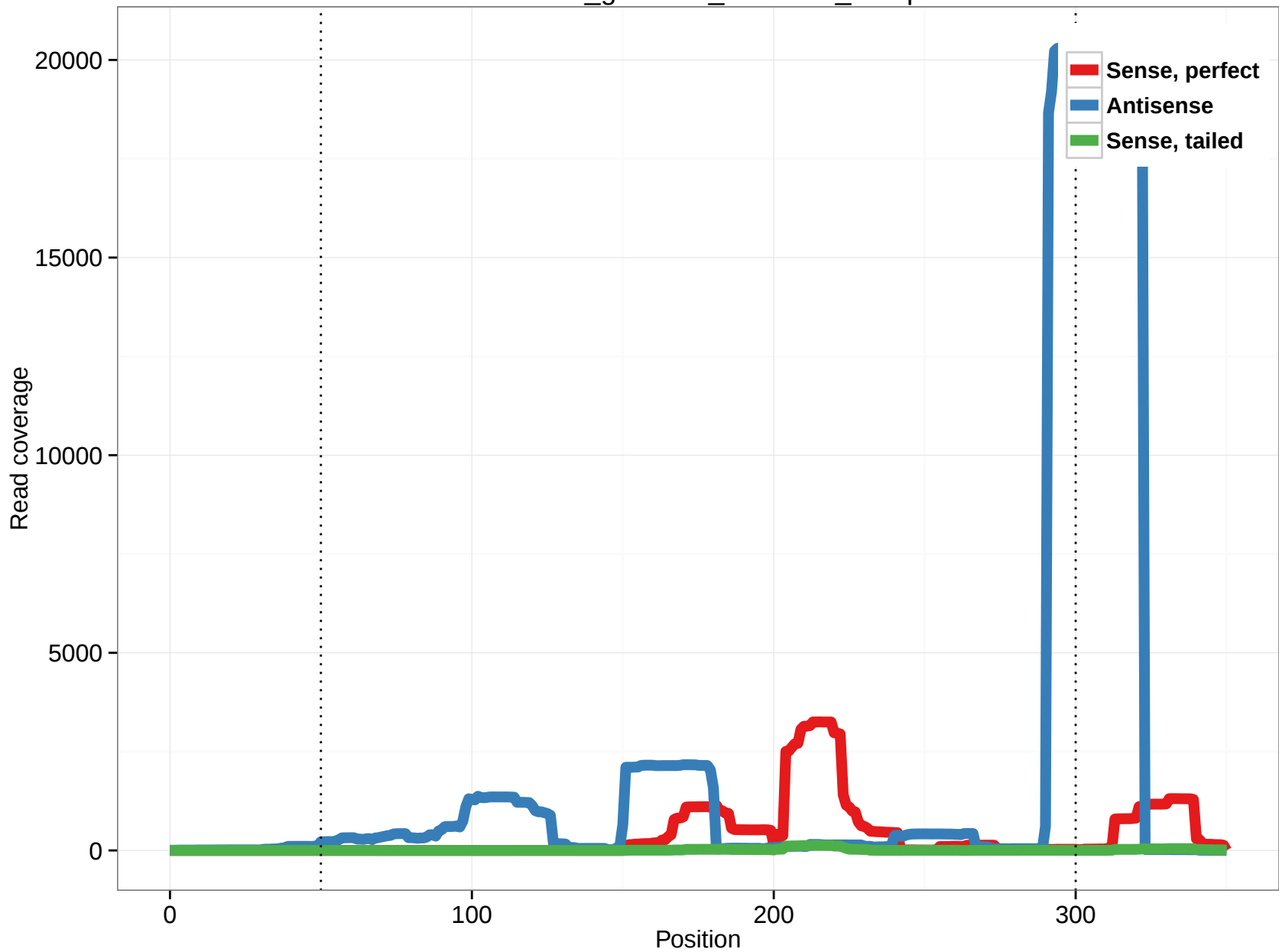
rheMac3_genscan_chr7.829_11.3p
