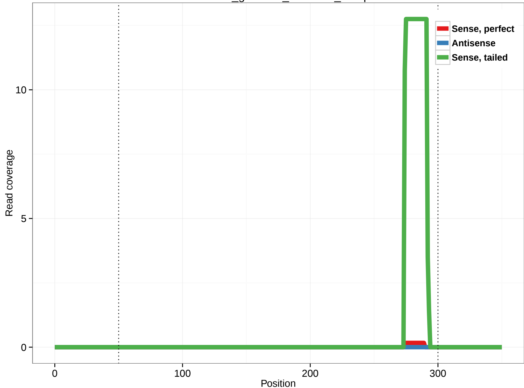
rheMac3_genscan_chr7.826_24.3p
