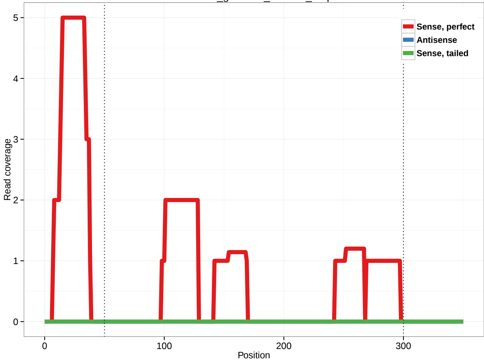
rheMac3_genscan_chr7.70_3.5p
