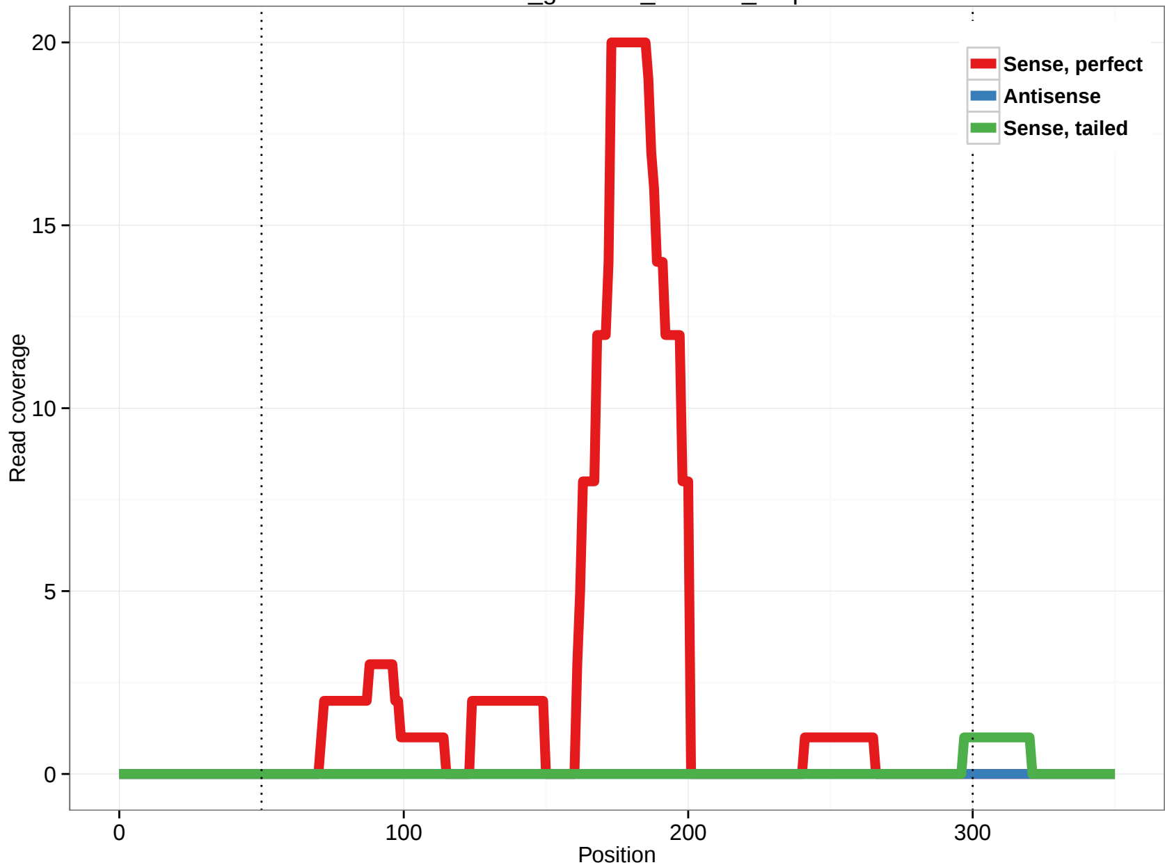
rheMac3_genscan_chr7.70_2.3p
