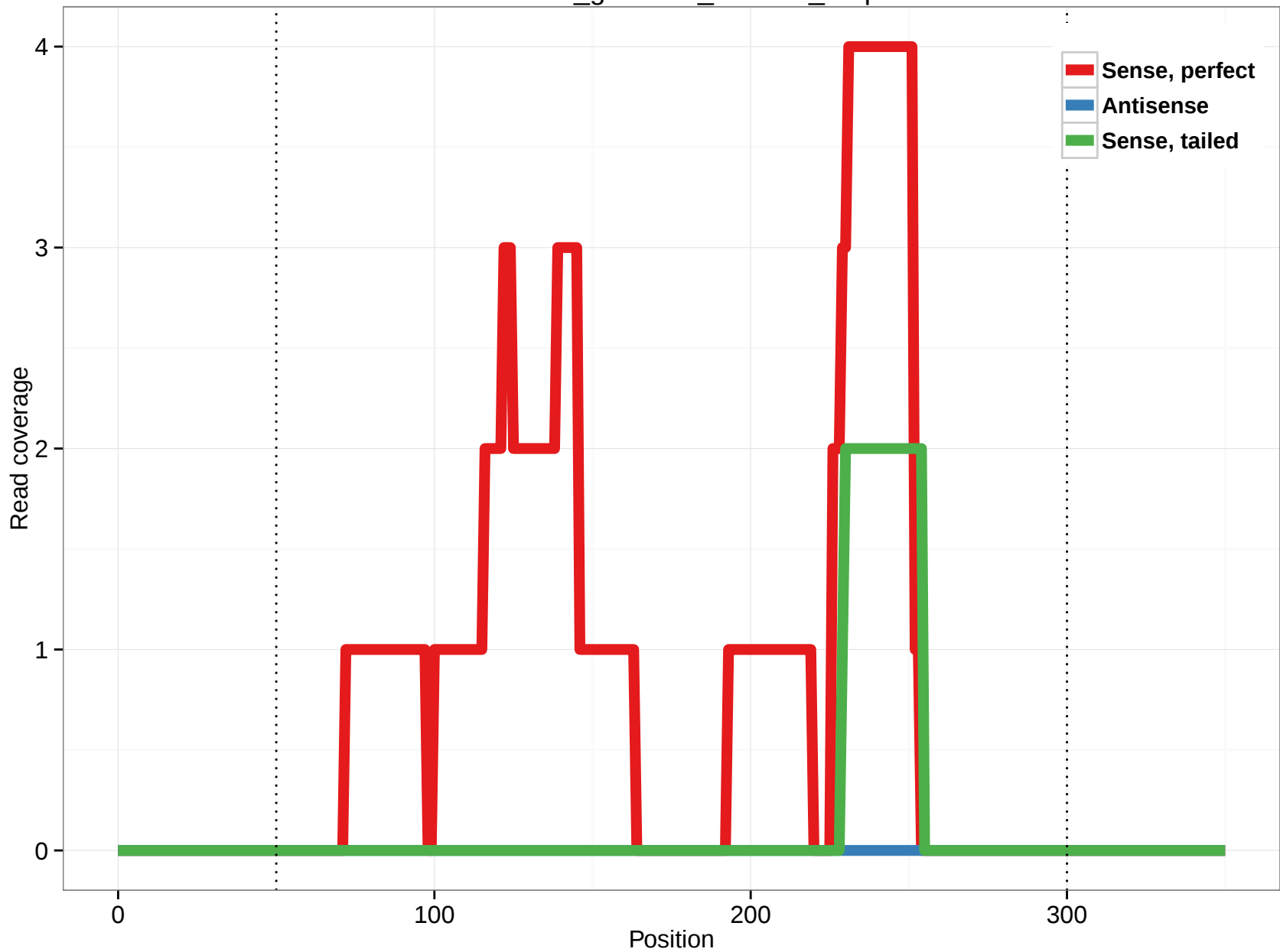
rheMac3_genscan_chr7.68_0.3p
