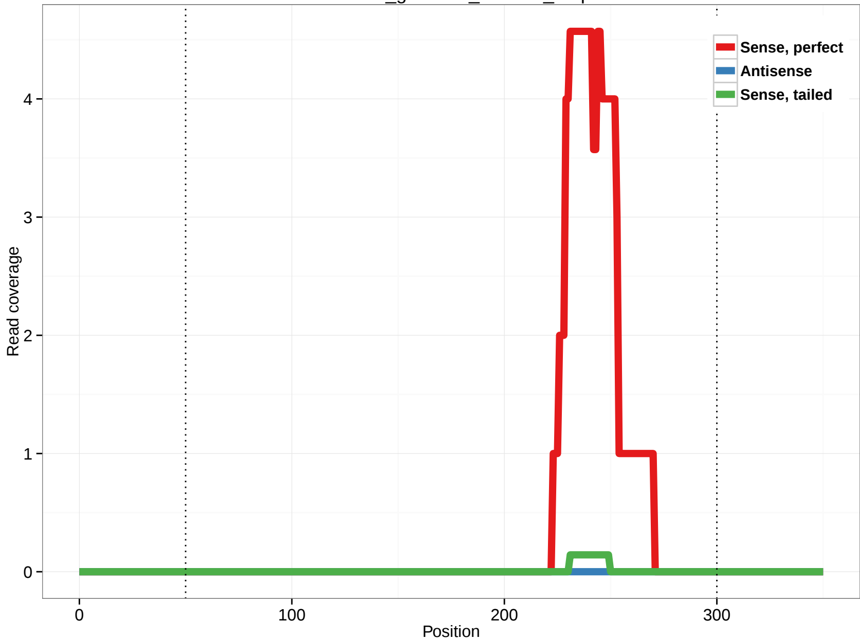
rheMac3_genscan_chr7.58_0.3p
