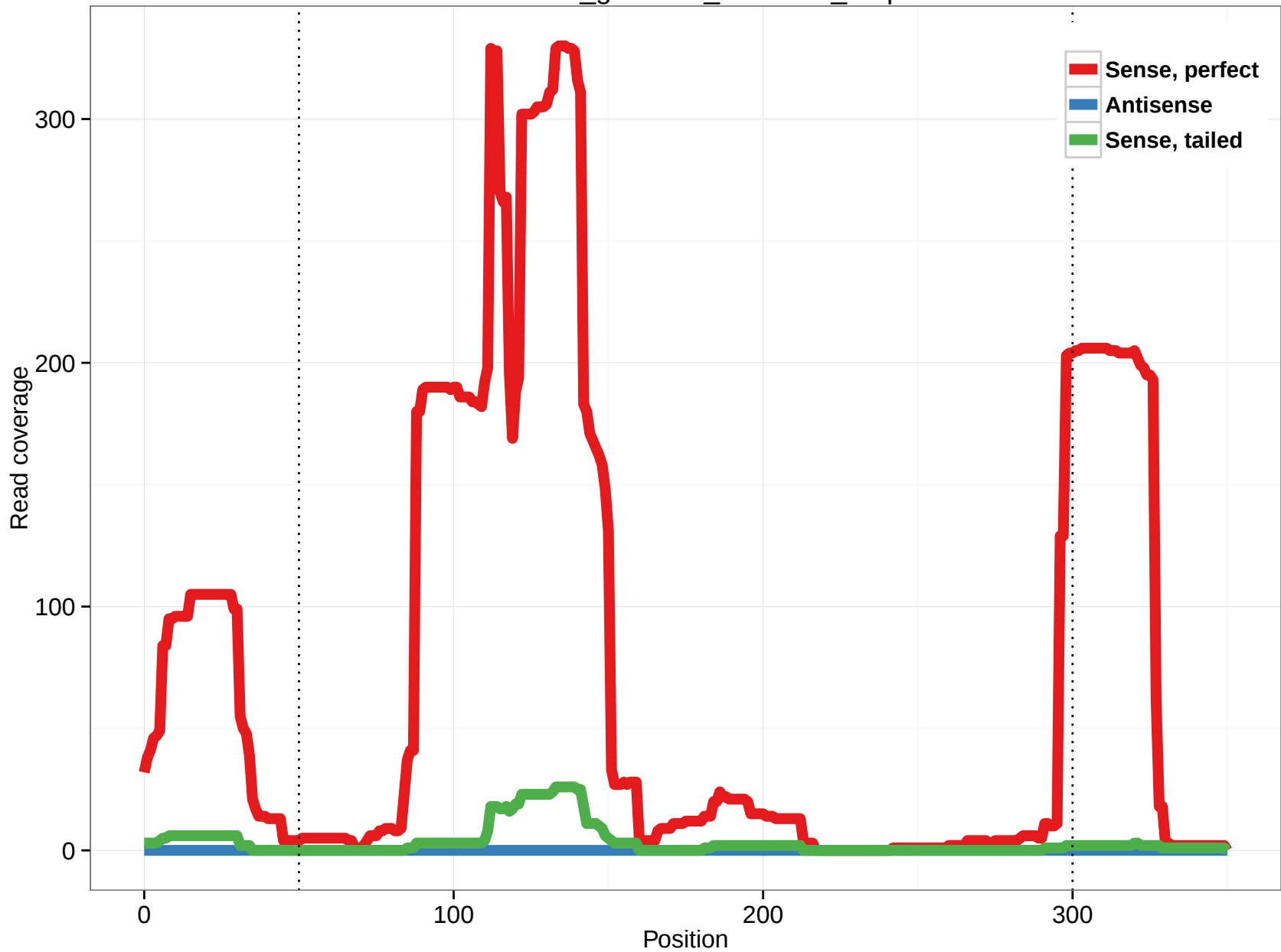
rheMac3_genscan_chr7.583_8.5p
