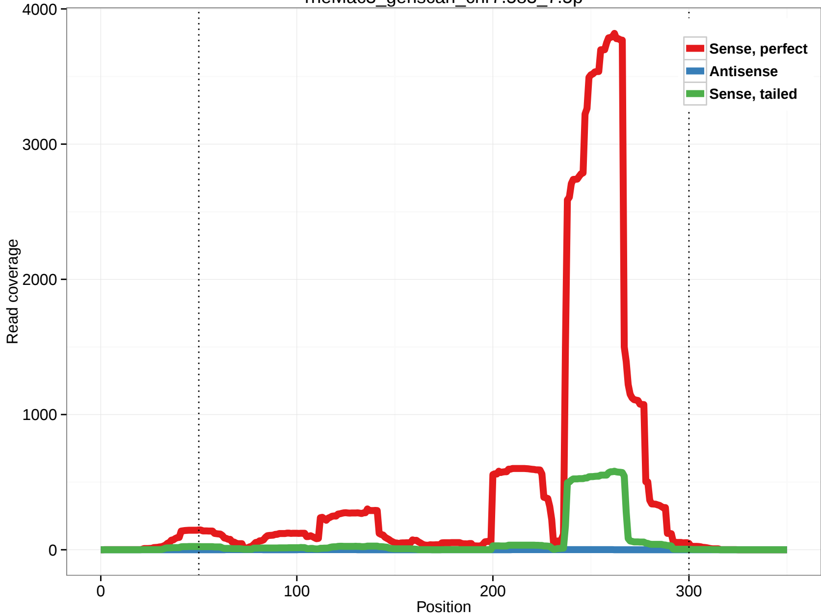
rheMac3_genscan_chr7.583_7.5p
