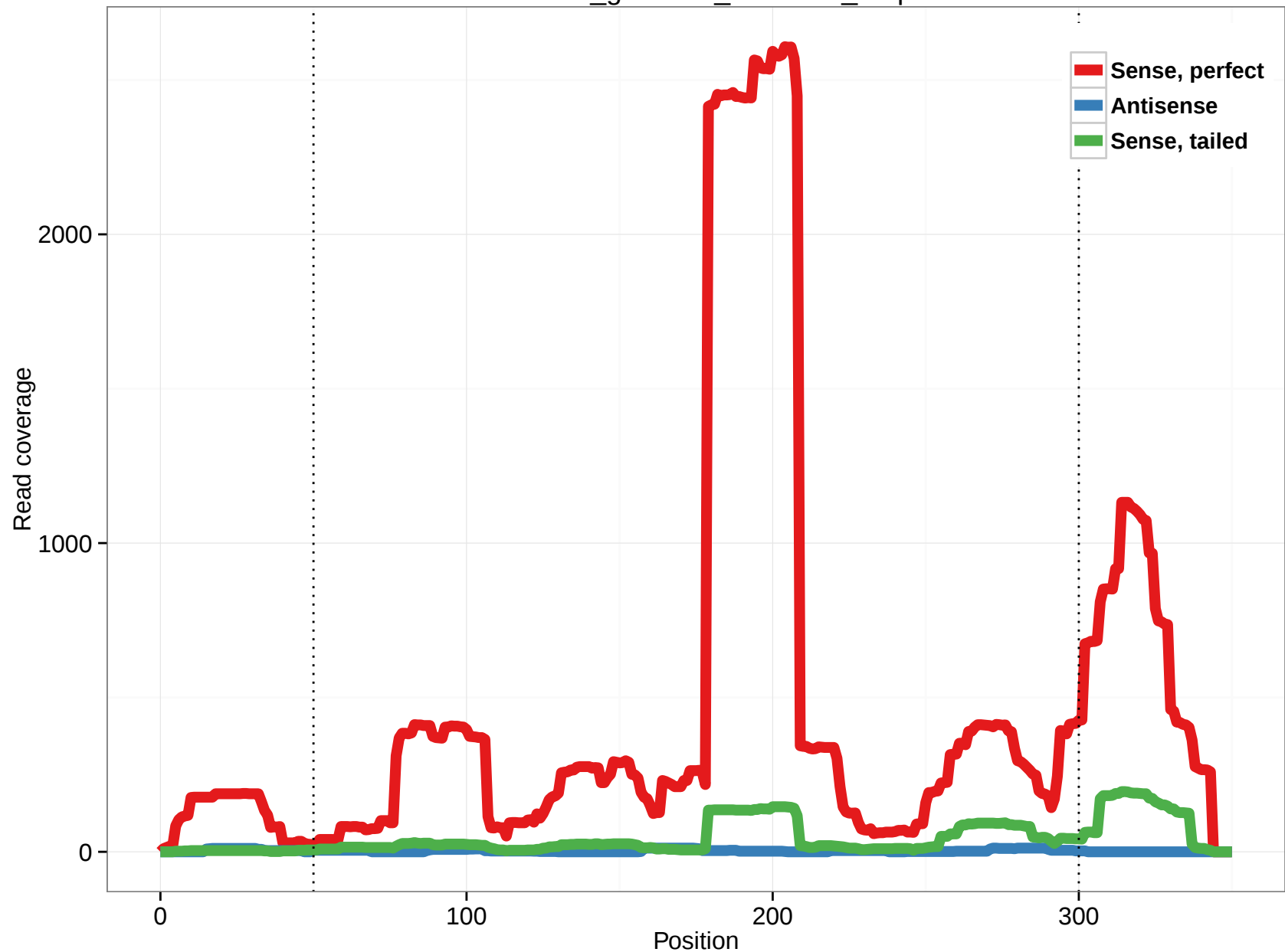
rheMac3_genscan_chr7.583_4.3p
