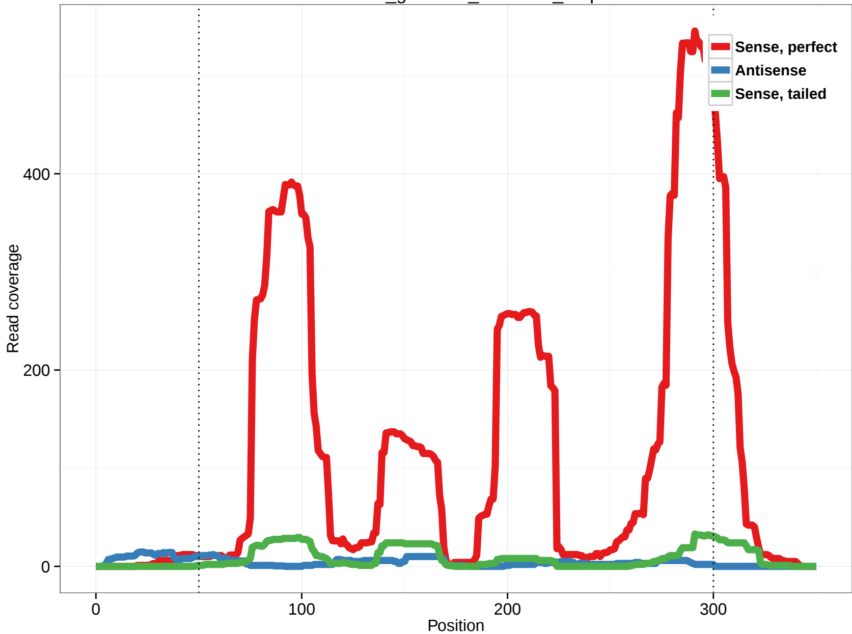
rheMac3_genscan_chr7.583_2.3p
