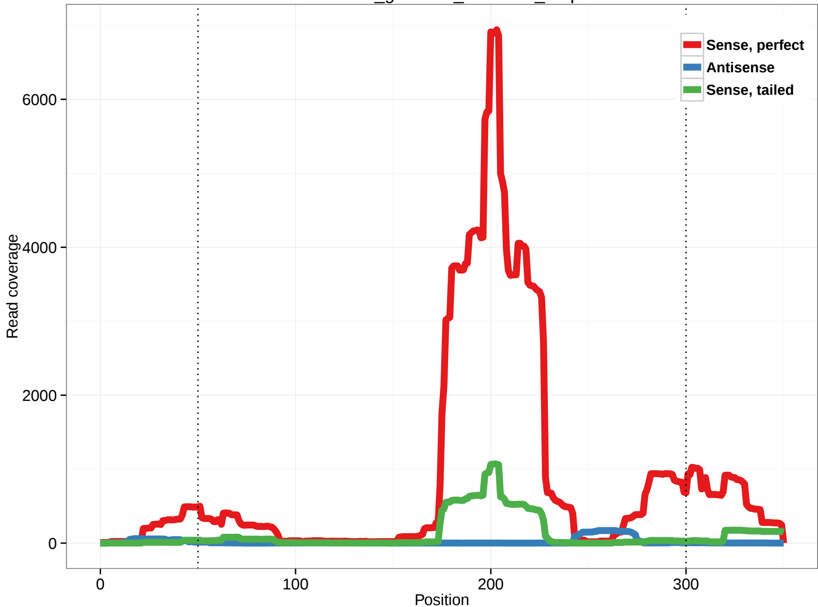
rheMac3_genscan_chr7.583_1.5p
