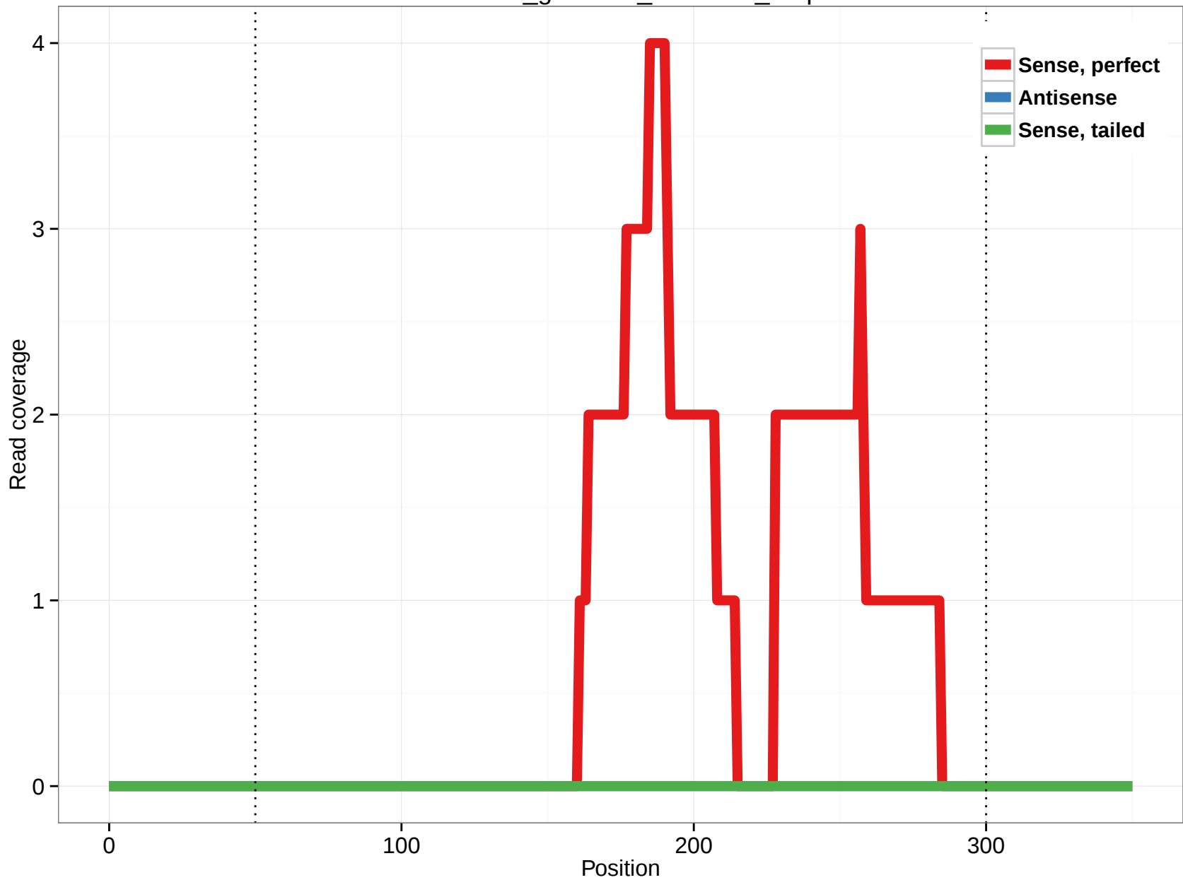
rheMac3_genscan_chr7.576_0.5p
