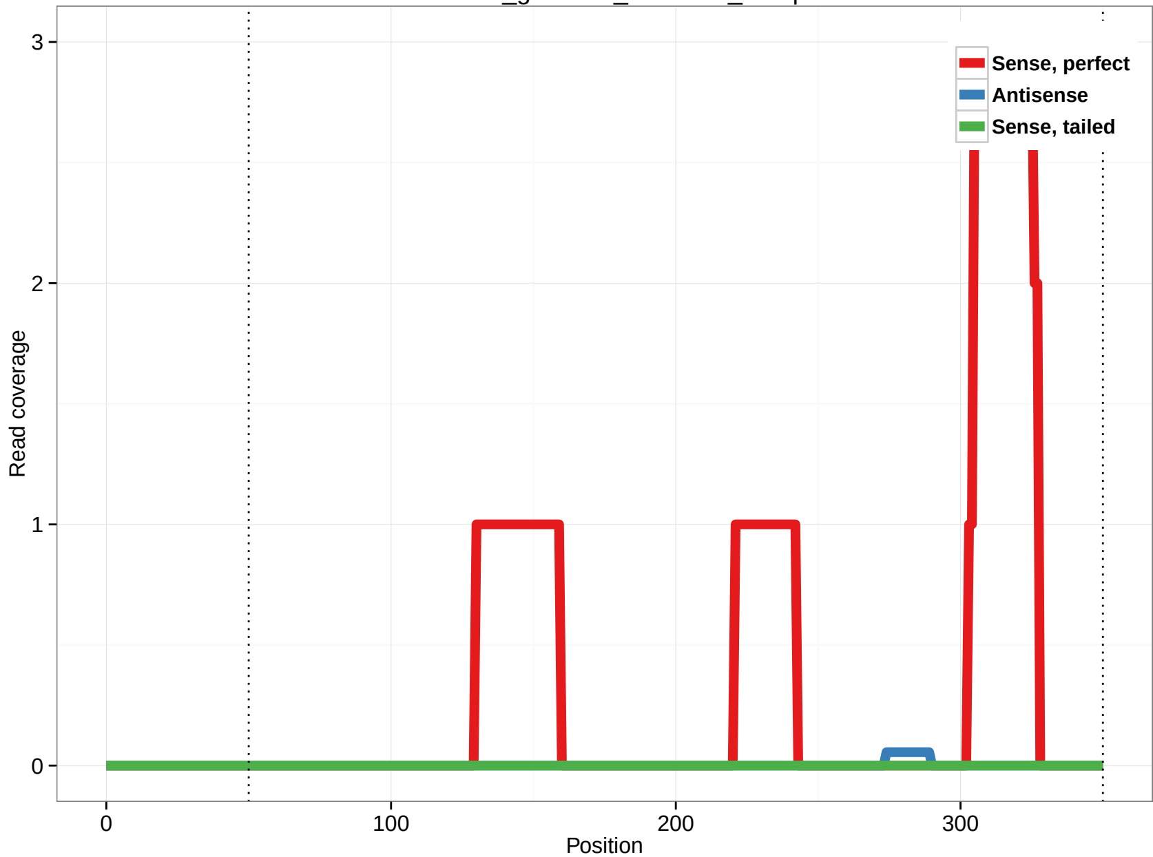
rheMac3_genscan_chr7.549_23.5p
