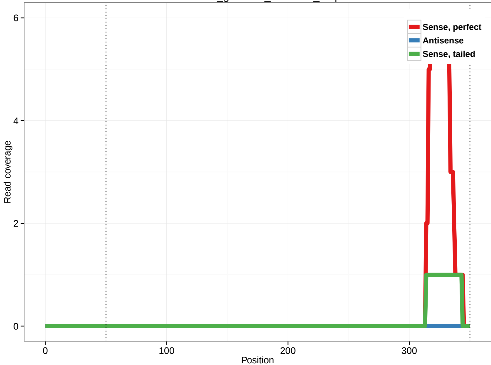
rheMac3_genscan_chr7.453_2.5p
