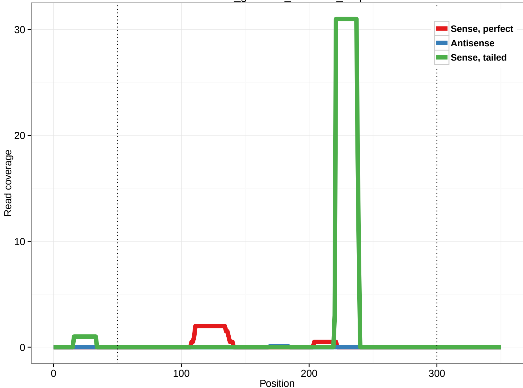
rheMac3_genscan_chr7.412_8.3p
