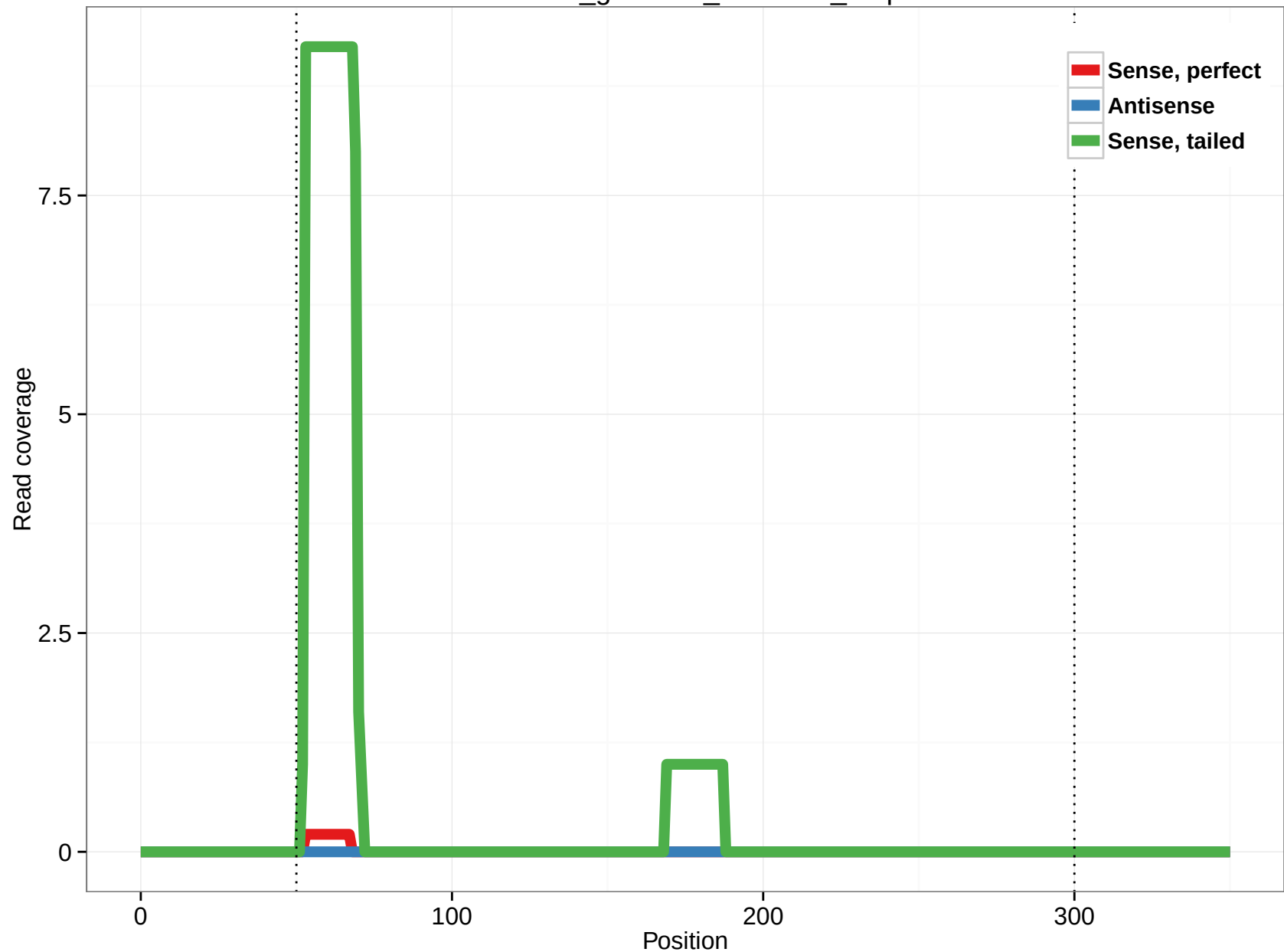
rheMac3_genscan_chr7.401_8.5p
