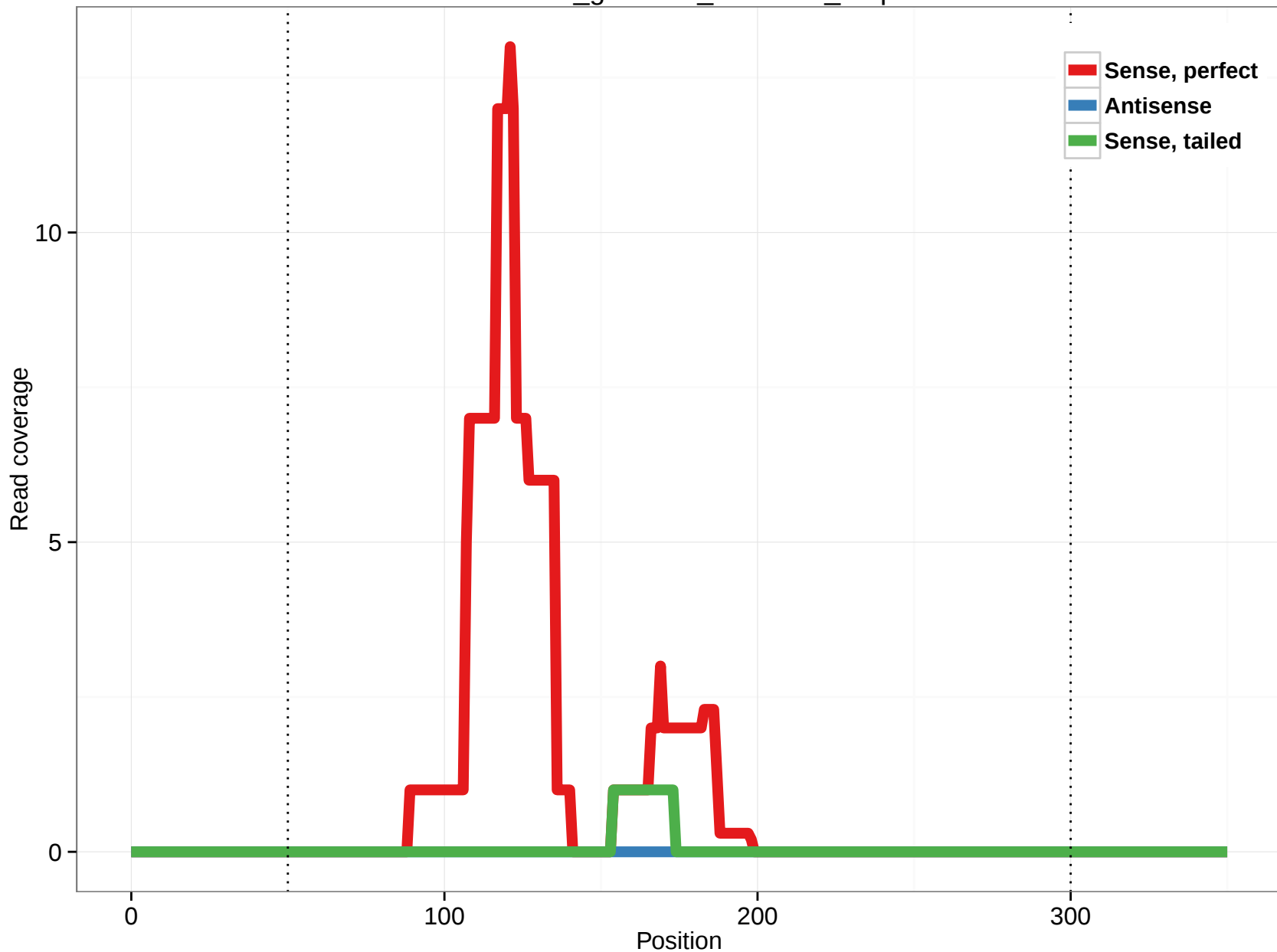
rheMac3_genscan_chr7.398_2.5p
