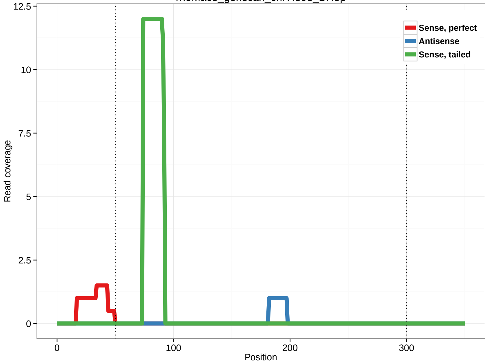
rheMac3_genscan_chr7.393_17.5p
