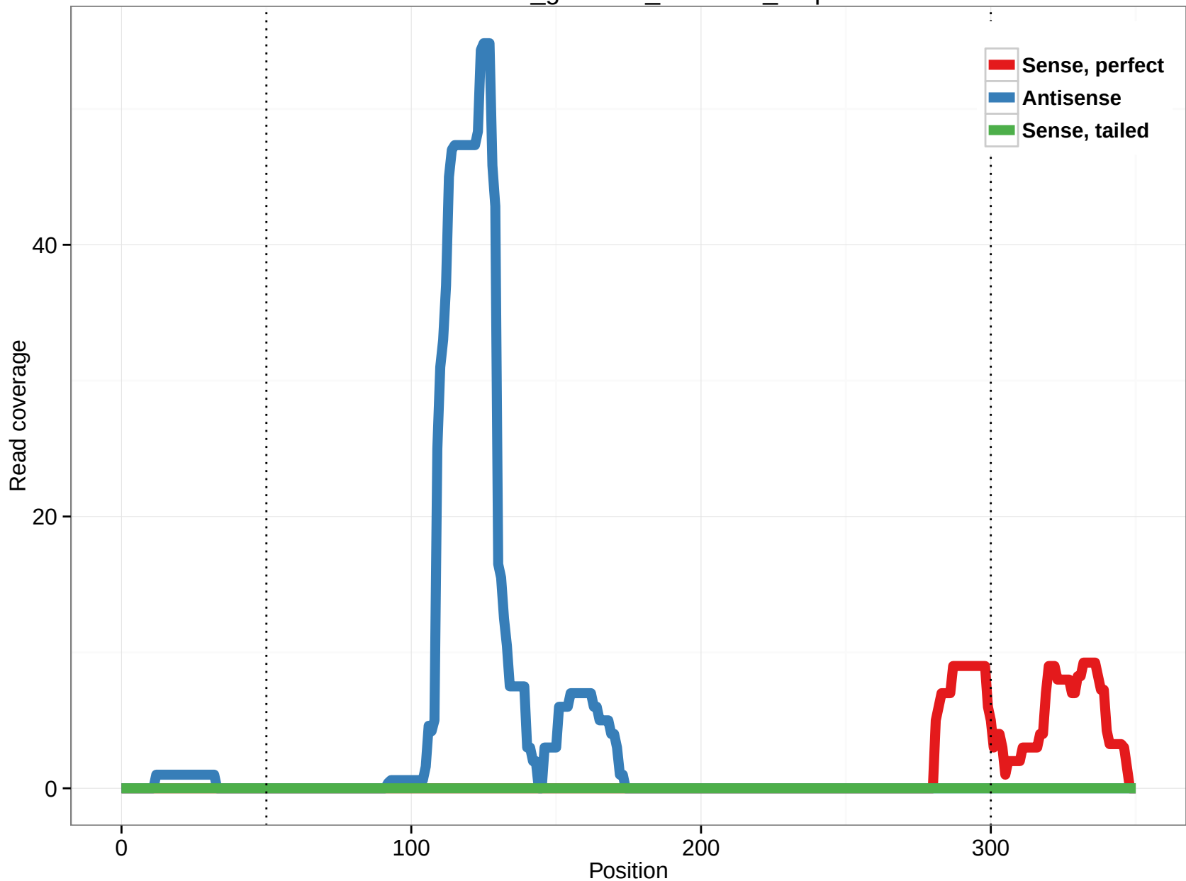
rheMac3_genscan_chr7.390_1.5p
