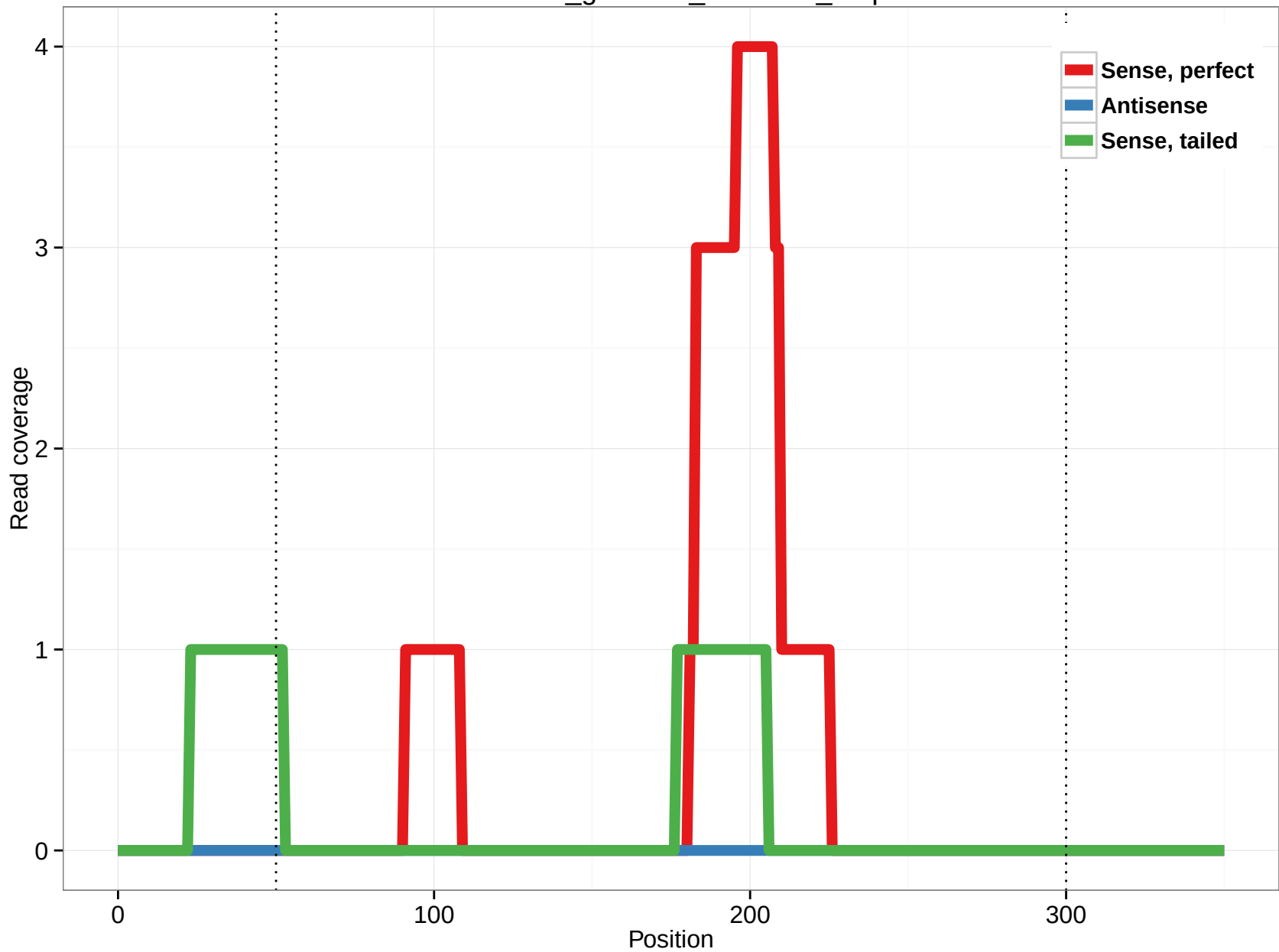
rheMac3_genscan_chr7.371_6.3p
