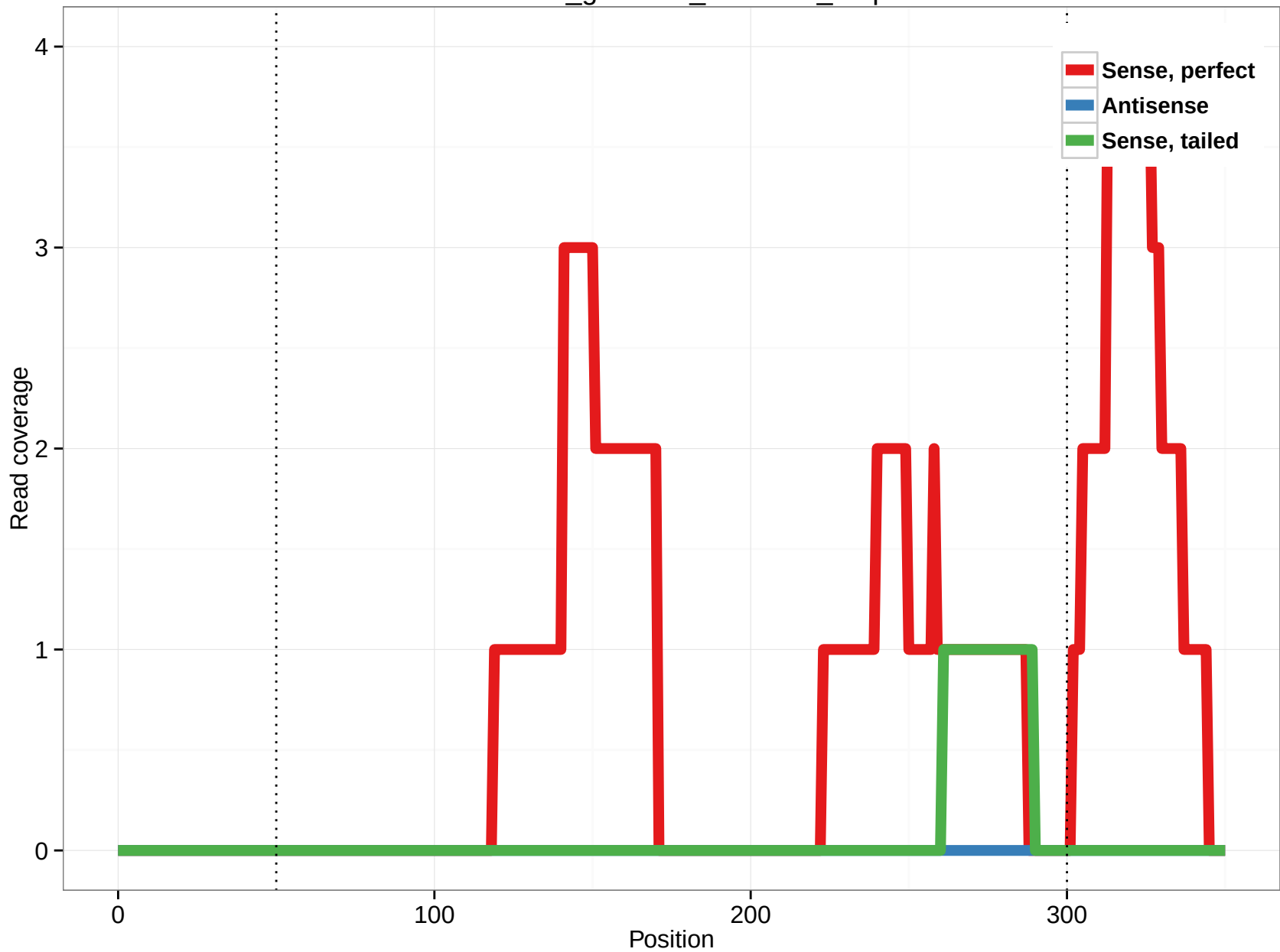
rheMac3_genscan_chr7.369_1.3p
