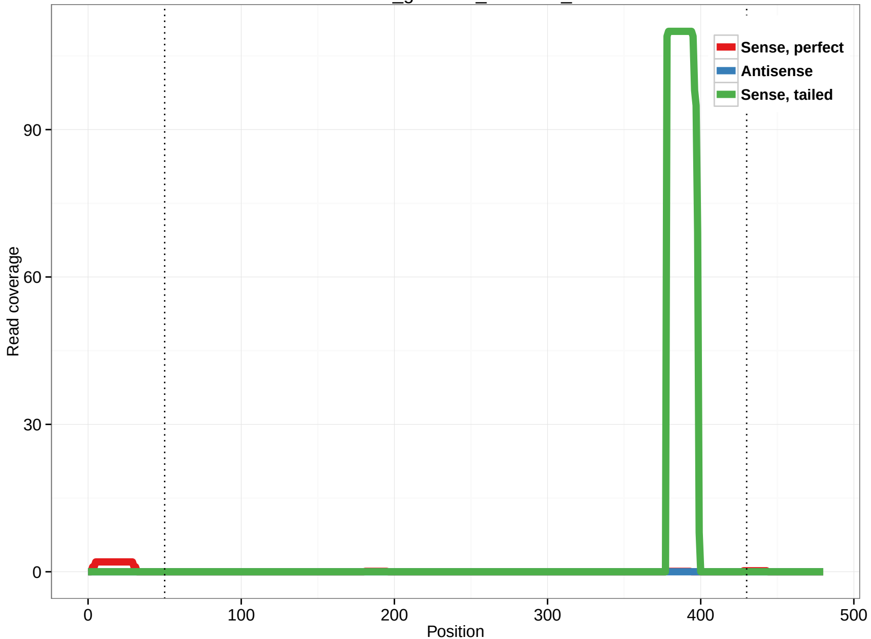
rheMac3_genscan_chr7.358_39
