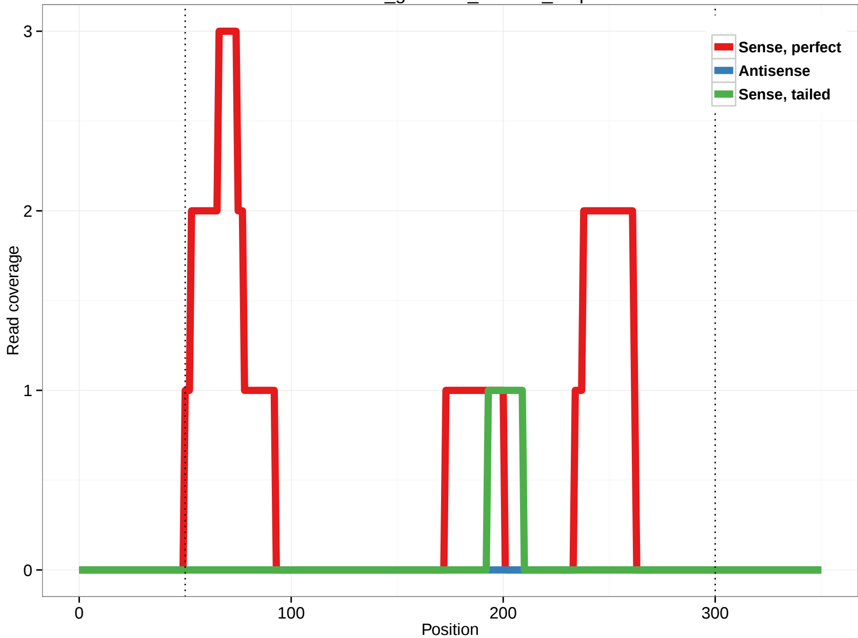
rheMac3_genscan_chr7.34_0.3p
