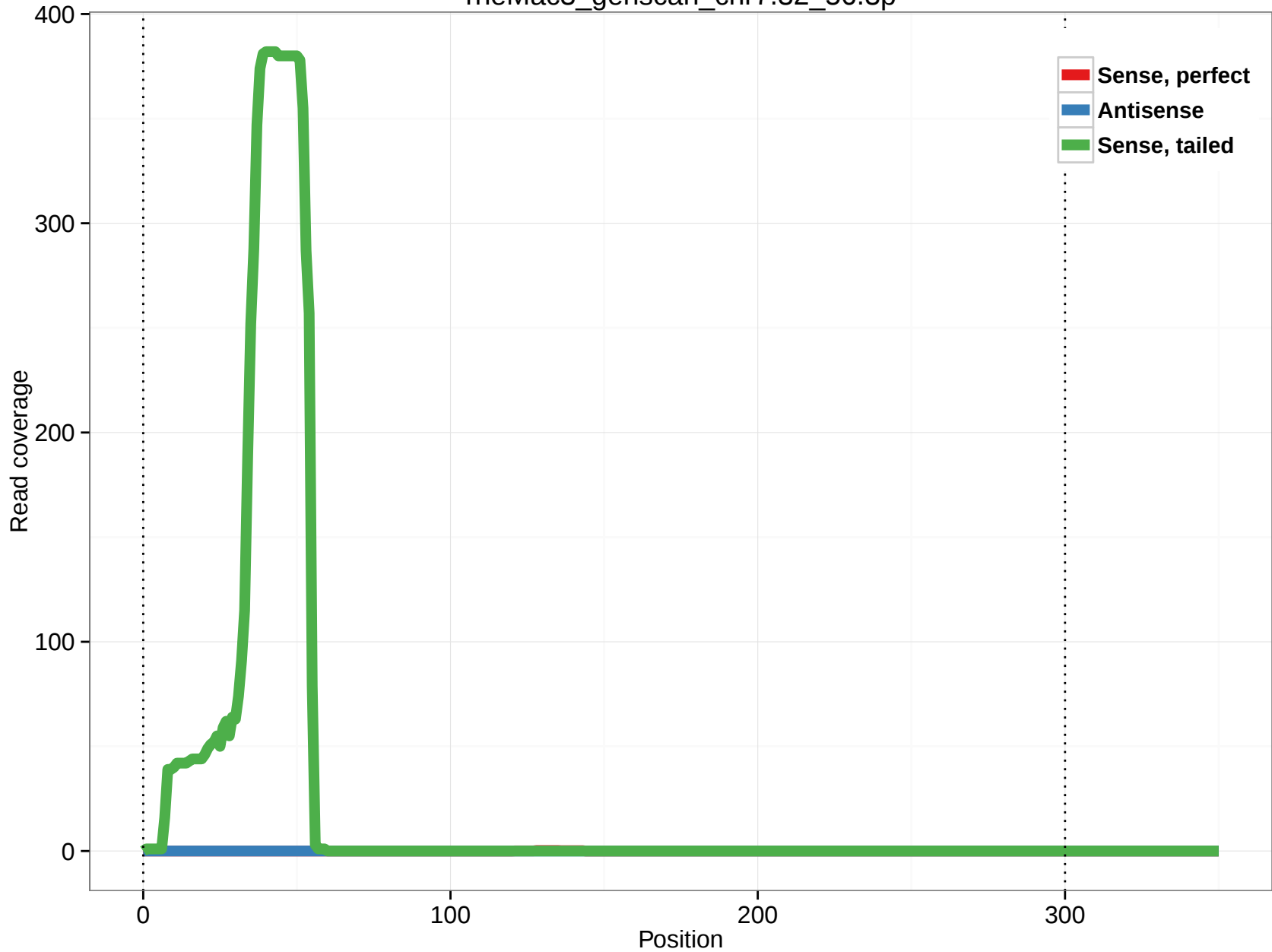
rheMac3_genscan_chr7.32_56.3p
