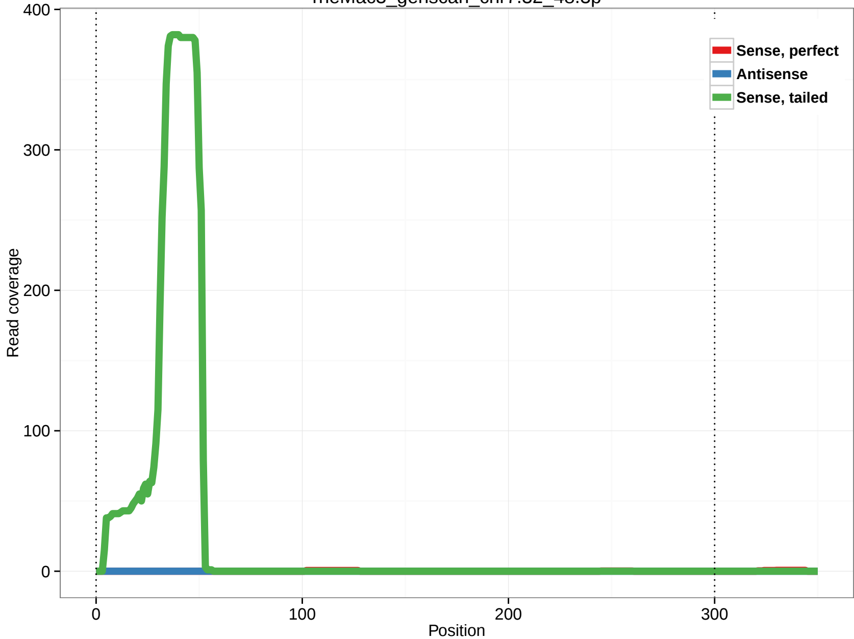
rheMac3_genscan_chr7.32_48.3p
