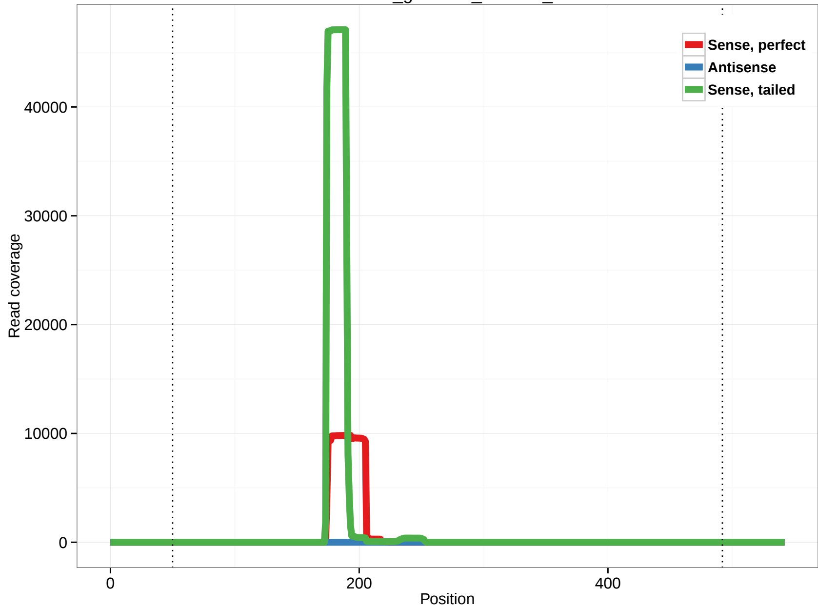
rheMac3_genscan_chr7.32_29
