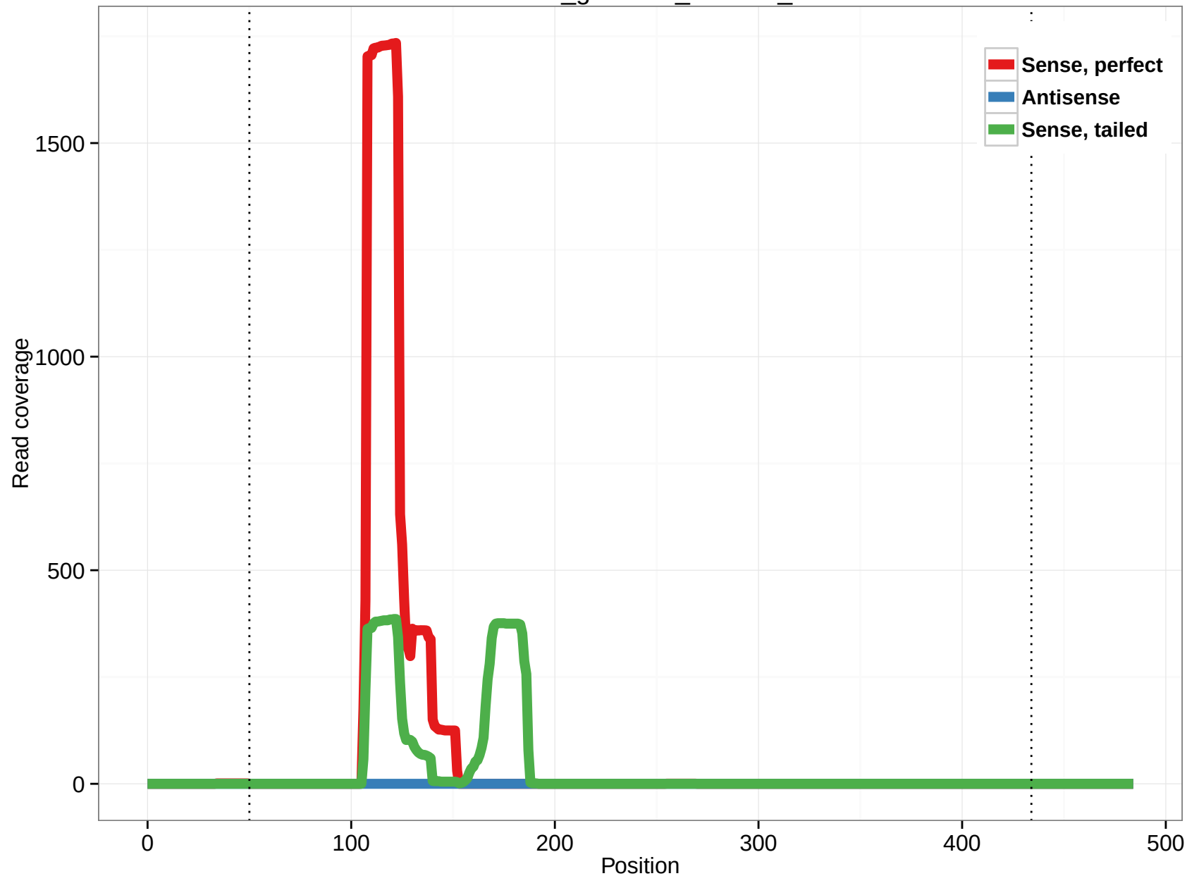
rheMac3_genscan_chr7.32_24
