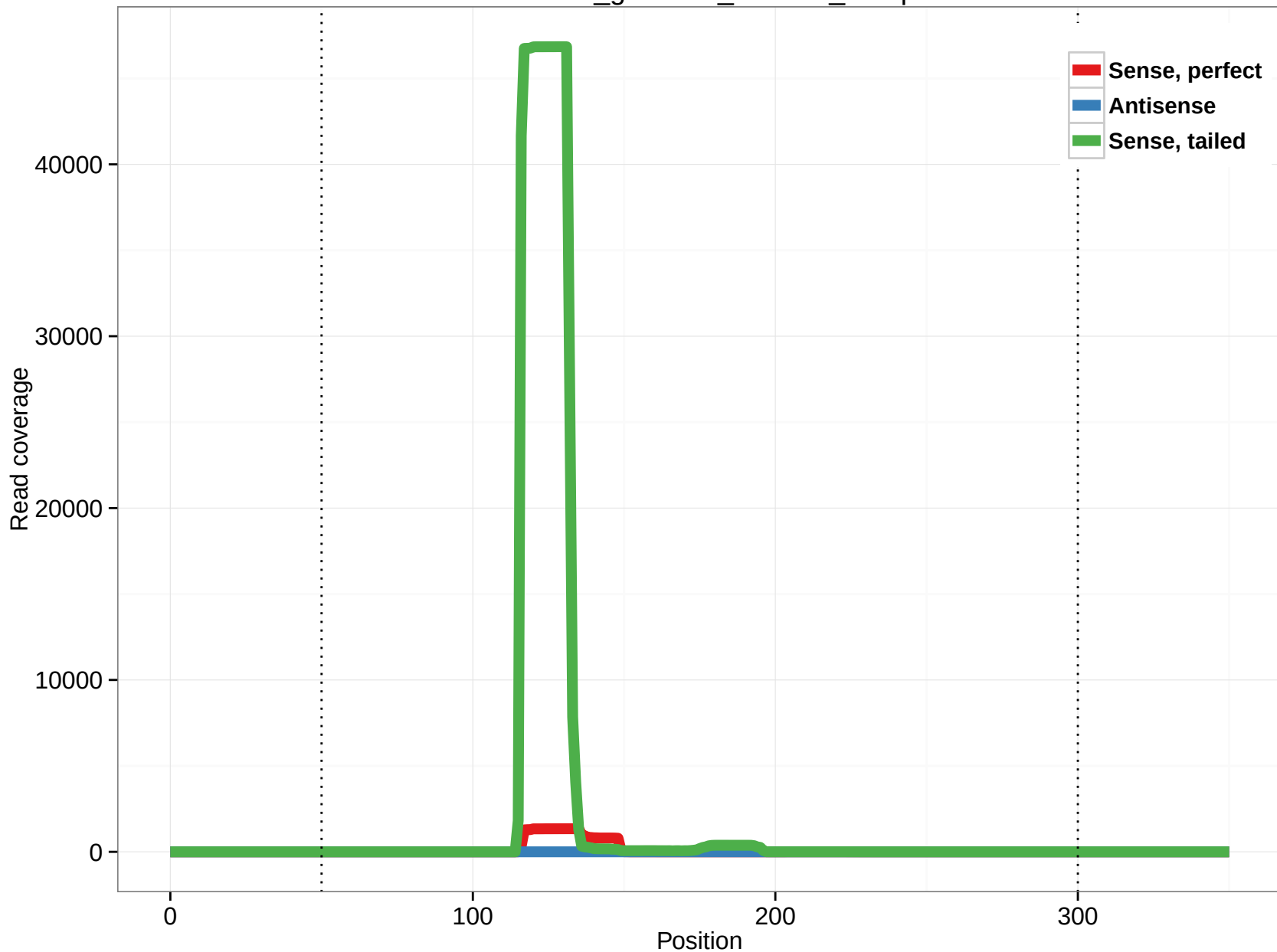
rheMac3_genscan_chr7.32_17.5p
