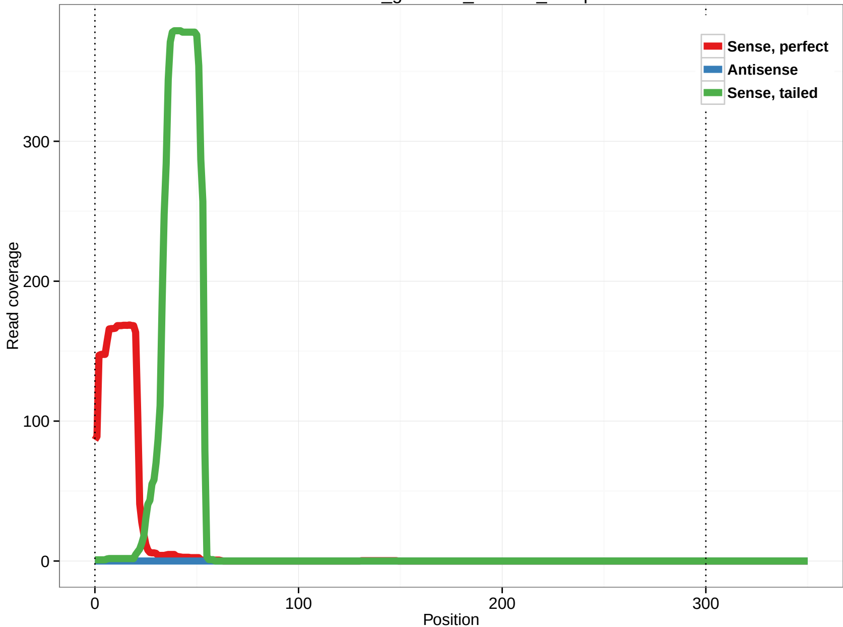
rheMac3_genscan_chr7.32_17.3p
