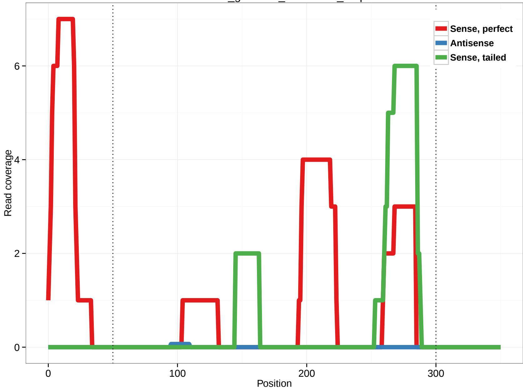
rheMac3_genscan_chr7.3265_8.5p
