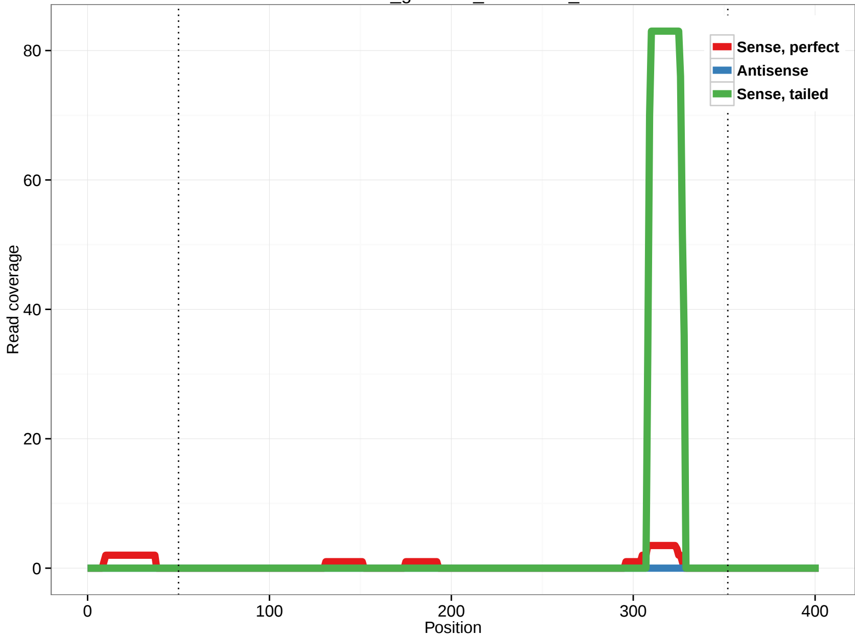
rheMac3_genscan_chr7.3255_4
