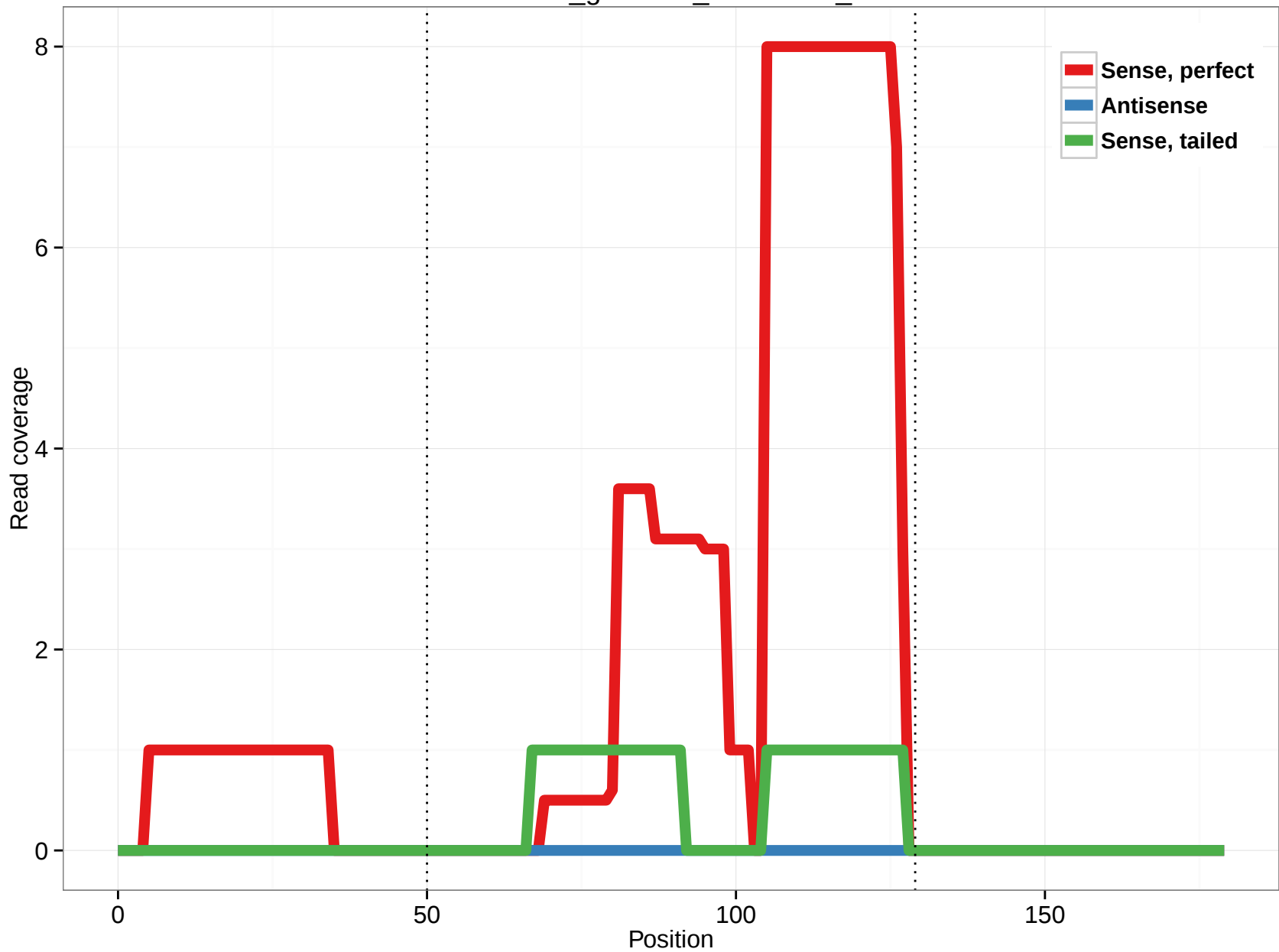
rheMac3_genscan_chr7.3249_11
