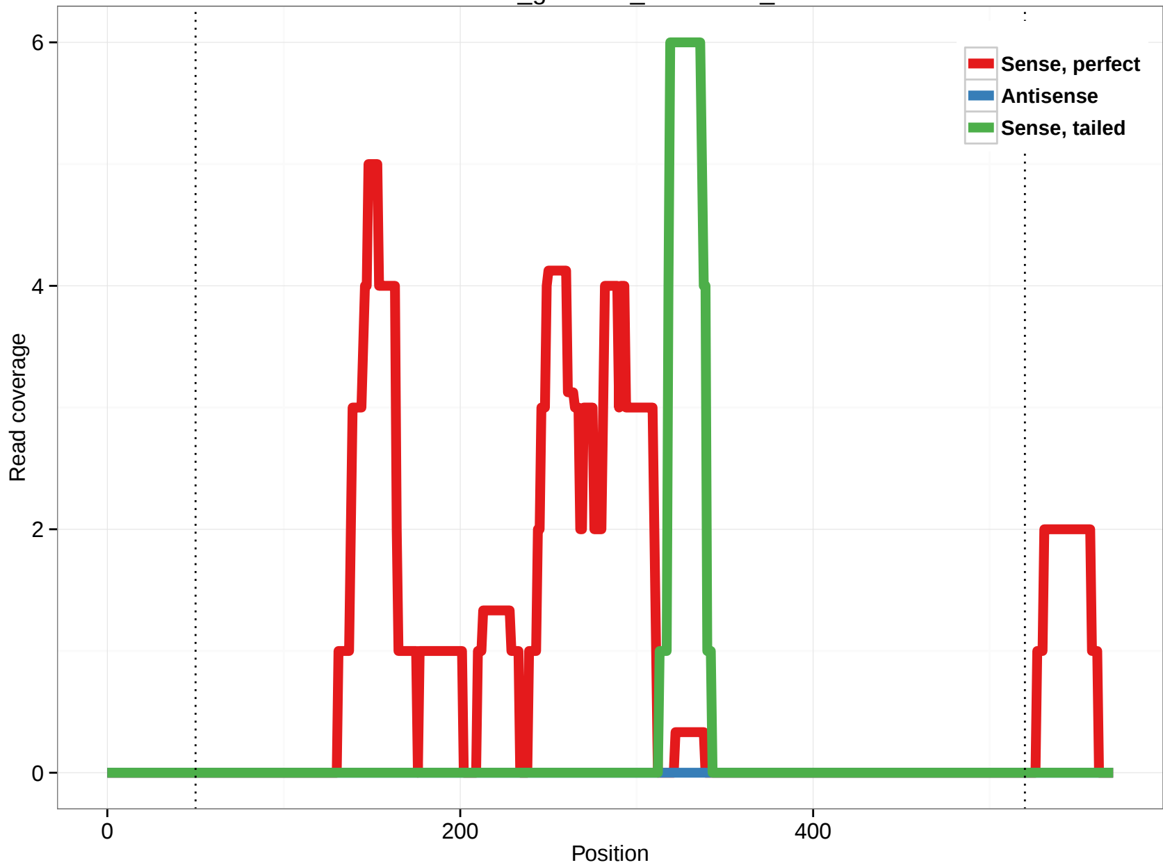
rheMac3_genscan_chr7.3216_19
