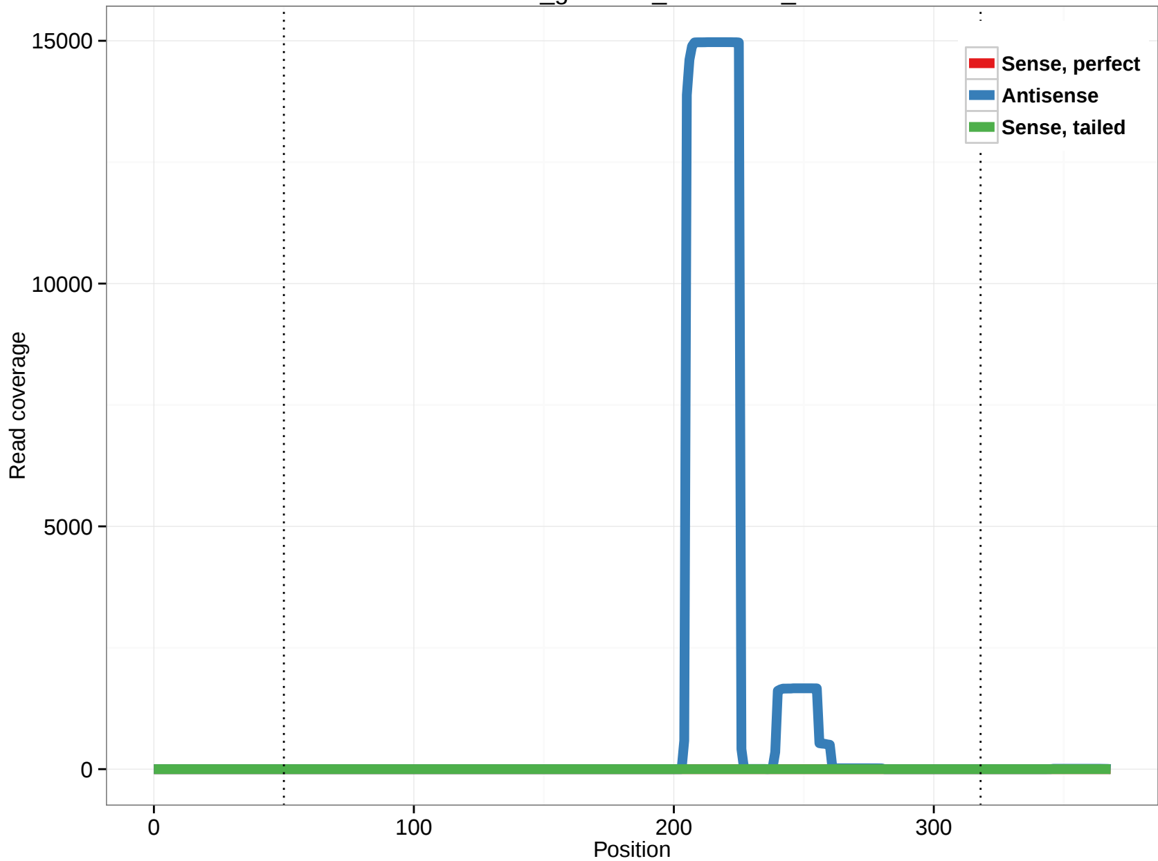
rheMac3_genscan_chr7.3189_10
