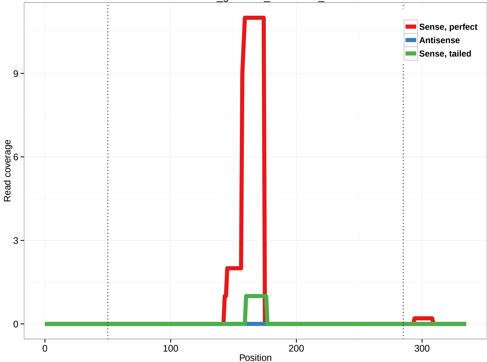
rheMac3_genscan_chr7.3188_12
