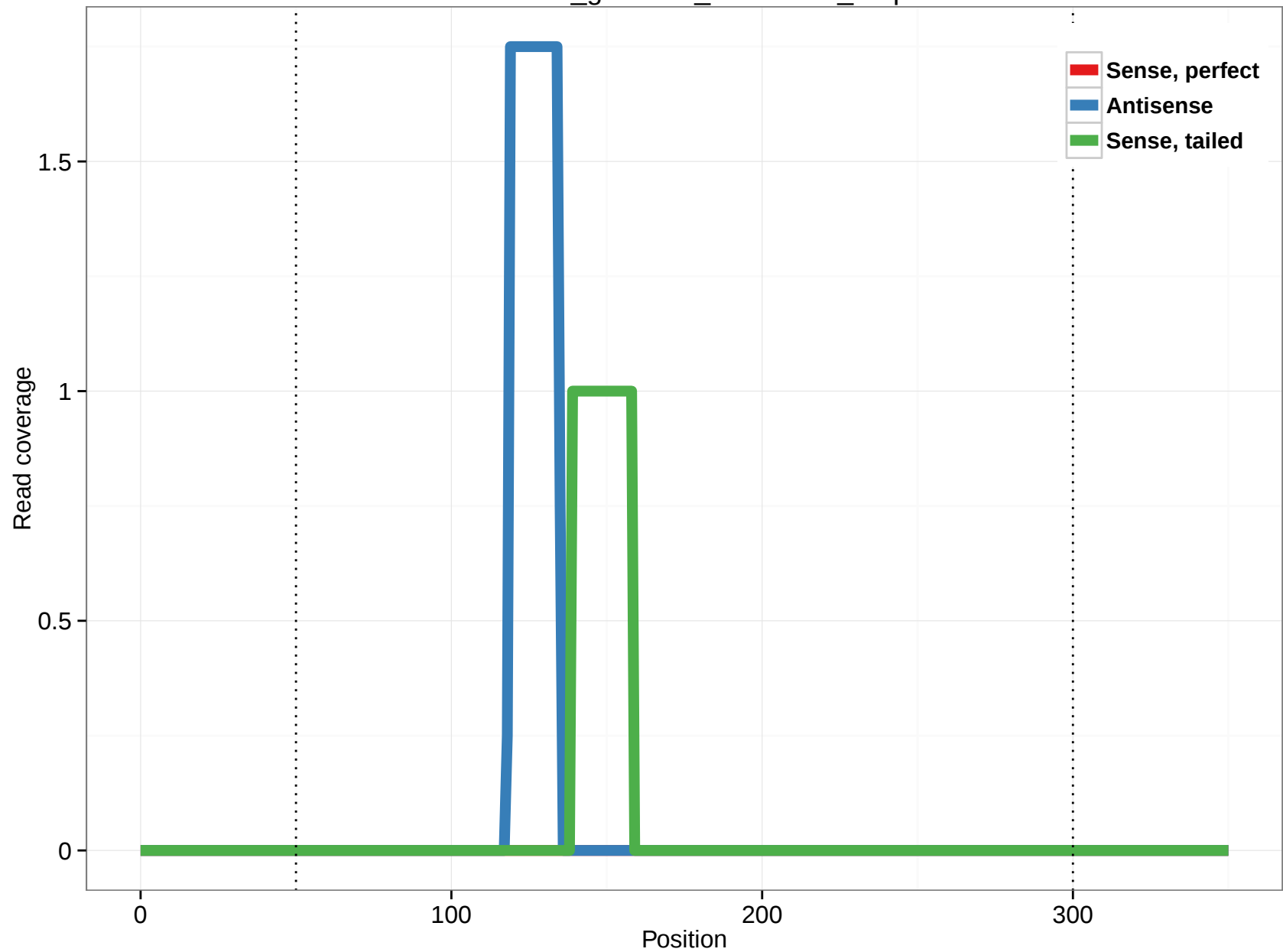
rheMac3_genscan_chr7.3171_0.5p
