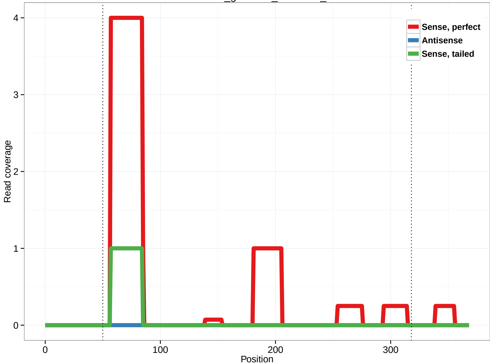
rheMac3_genscan_chr7.314_0
