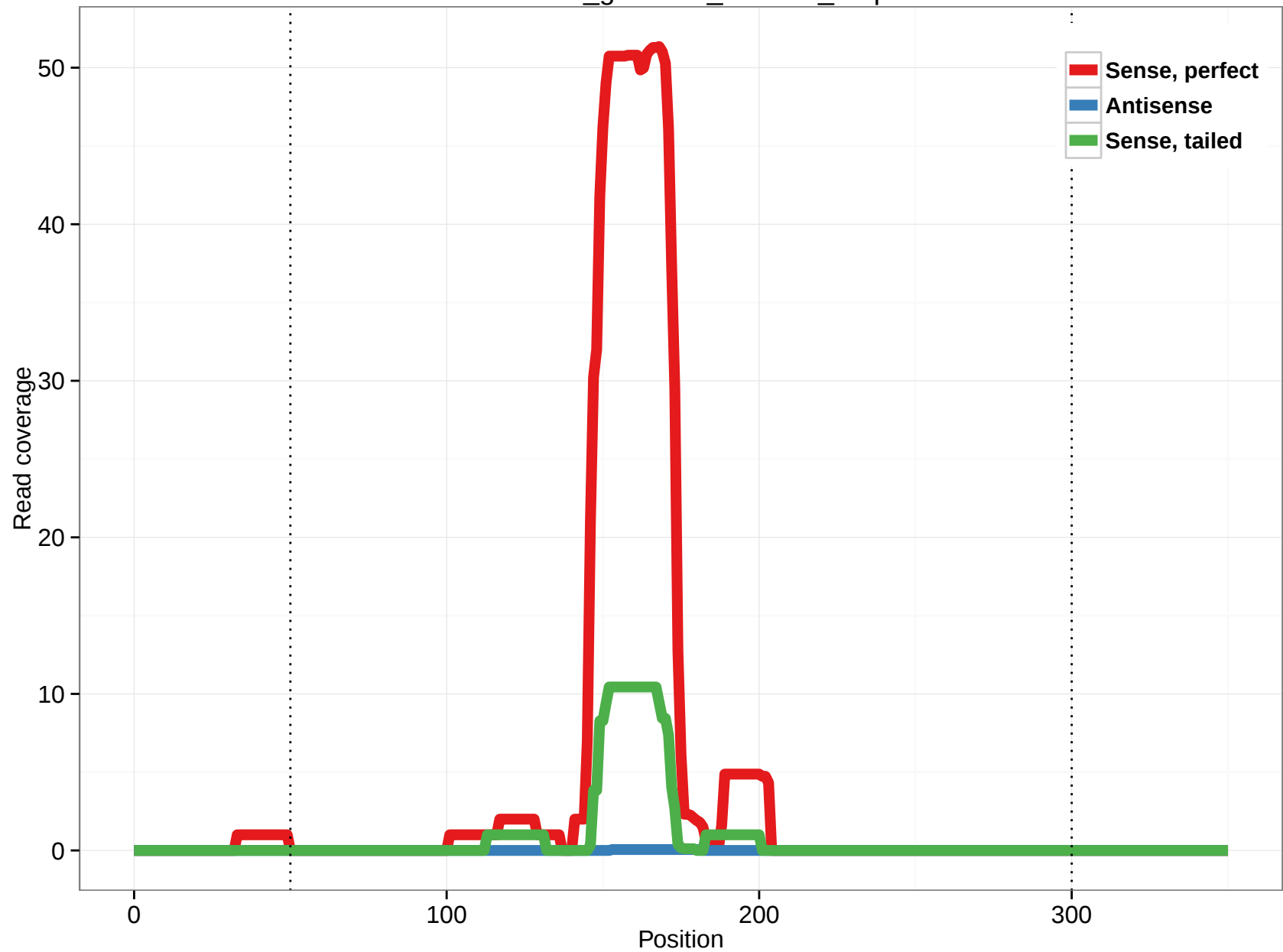
rheMac3_genscan_chr7.30_8.5p
