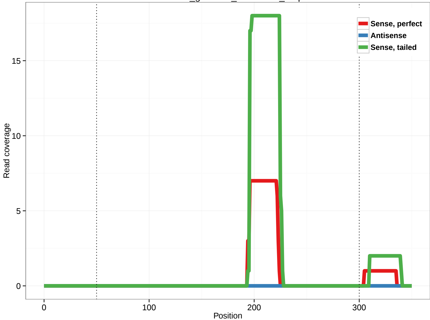
rheMac3_genscan_chr7.3087_1.5p
